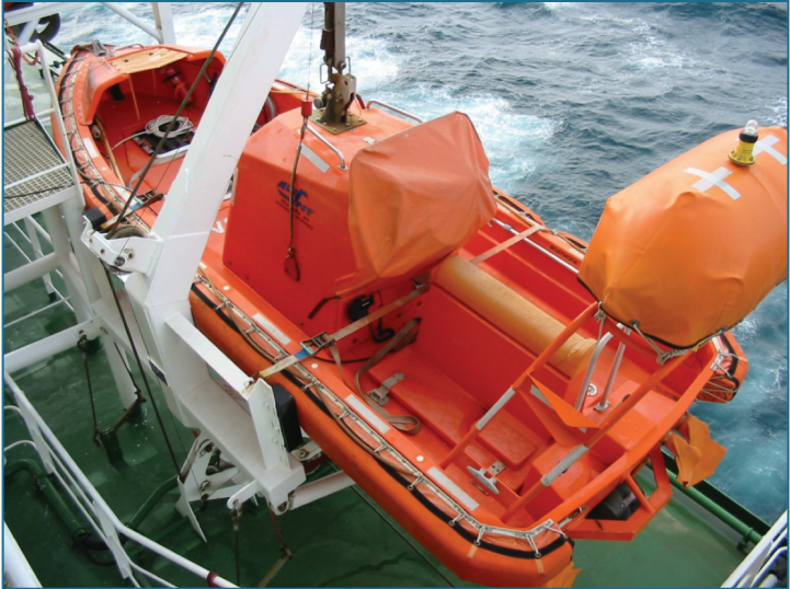
Fig. 10 Rescue boat in stowed position
