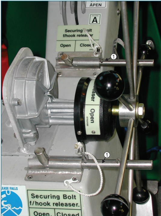
Fig. 9 Boat release handle
