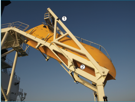
Fig. 8 Free-fall lifeboat in stowed position
