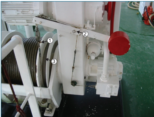
Fig. 2 Arrangement for brake remote release cable
