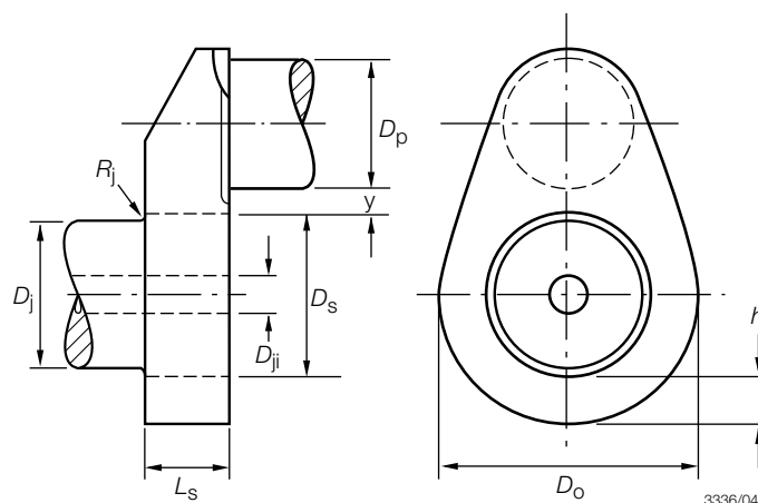
Figure 2.3.5 Crank throw of semi-built crankshaft
