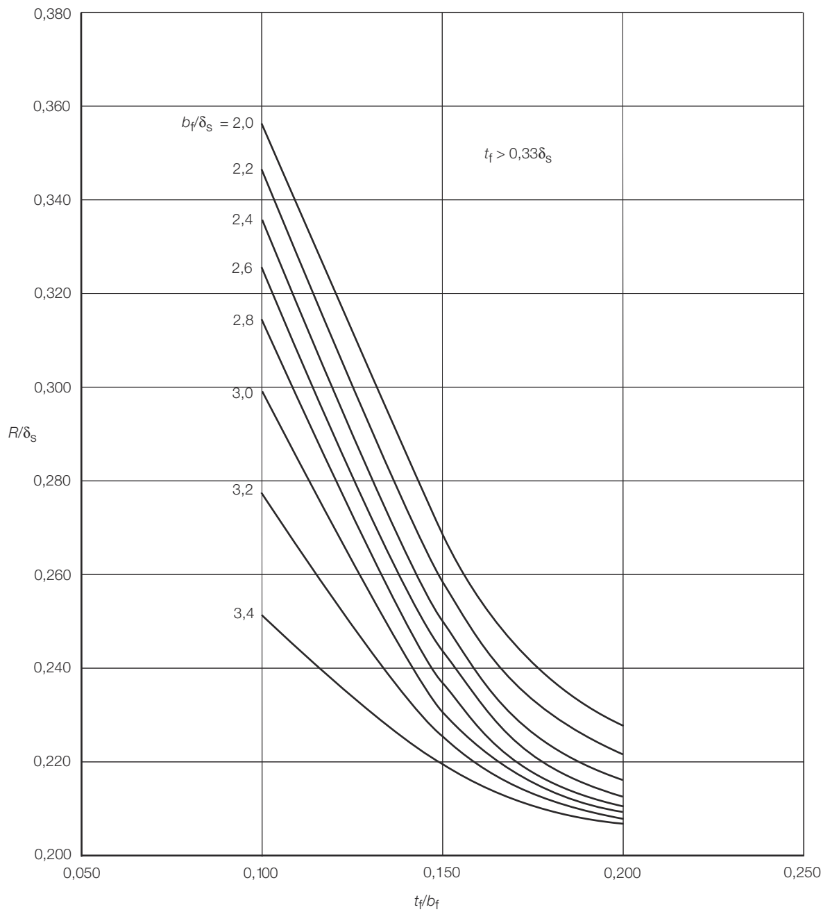
Figure 13.2.7 Rudder stock horizontal flange fillet radius for spade rudders
