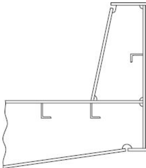
Figure 11.5.2 Example for the extent of coaming plates
