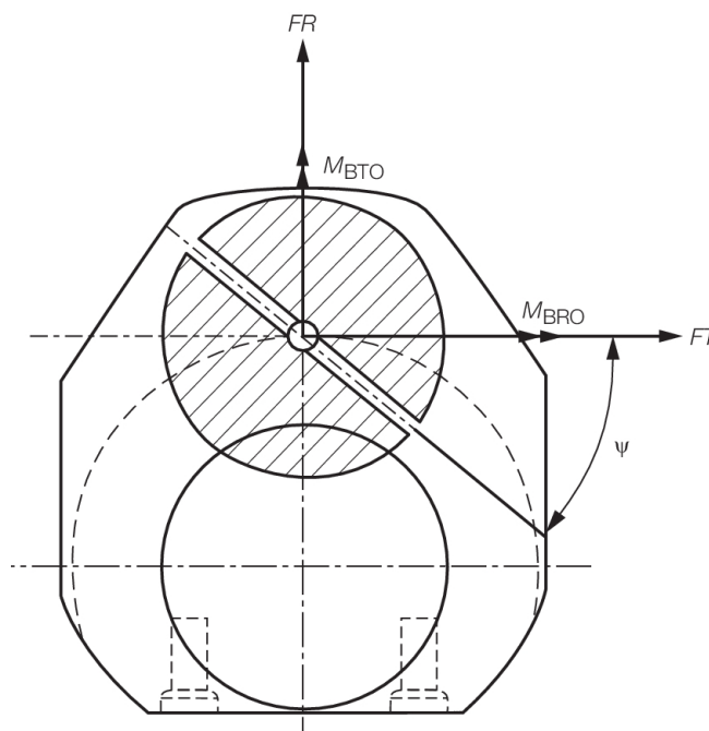
Figure 2.3.4 Crankpin section through the oil bore
