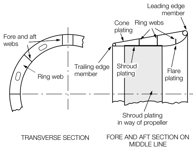
Figure 13.3.1 Nozzle construction
