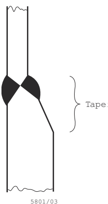
5801/03 Figure 4.6.3 Tapered plates
