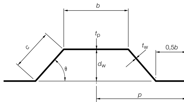
Figure 3.3.1 Corrugation dimensions
