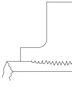
Figure 12.2.1 Screwed-on flange
