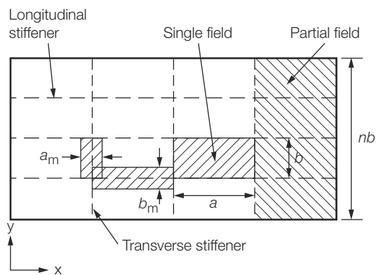
Figure 11.2.4 General arrangement of panel
