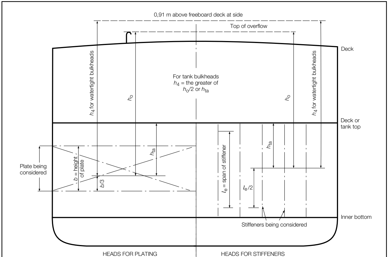
(a) Heads for watertight and deep tank bulkheads in intact condition
