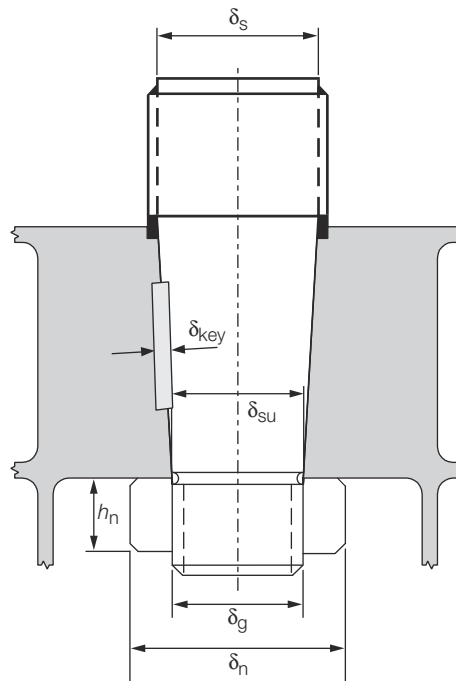
Figure 13.2.9 Conical coupling
