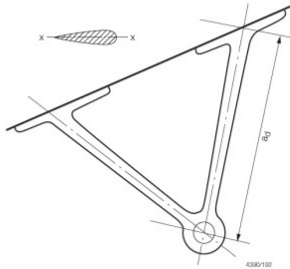
Figure 6.7.5 Double arm shaft bracket
