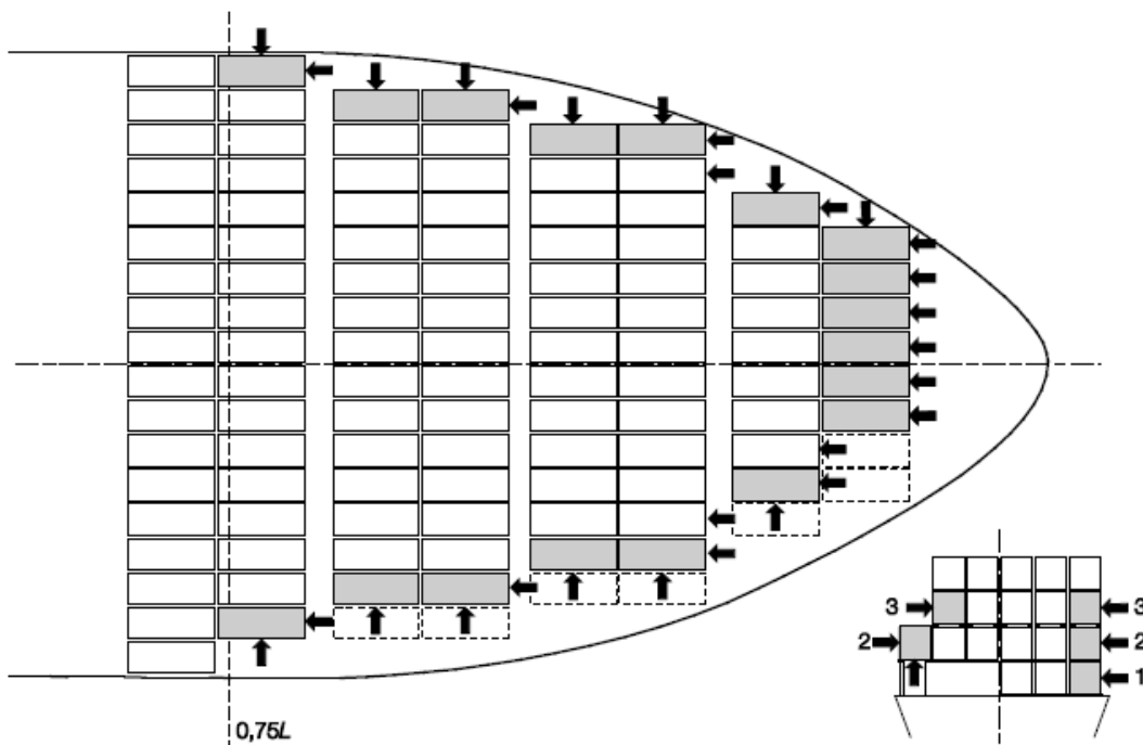
(b) Green sea loading on lowest three tiers only – No effective breakwater
