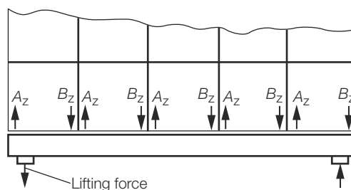
Figure 8.11.3 Lifting forces at a hatch cover
