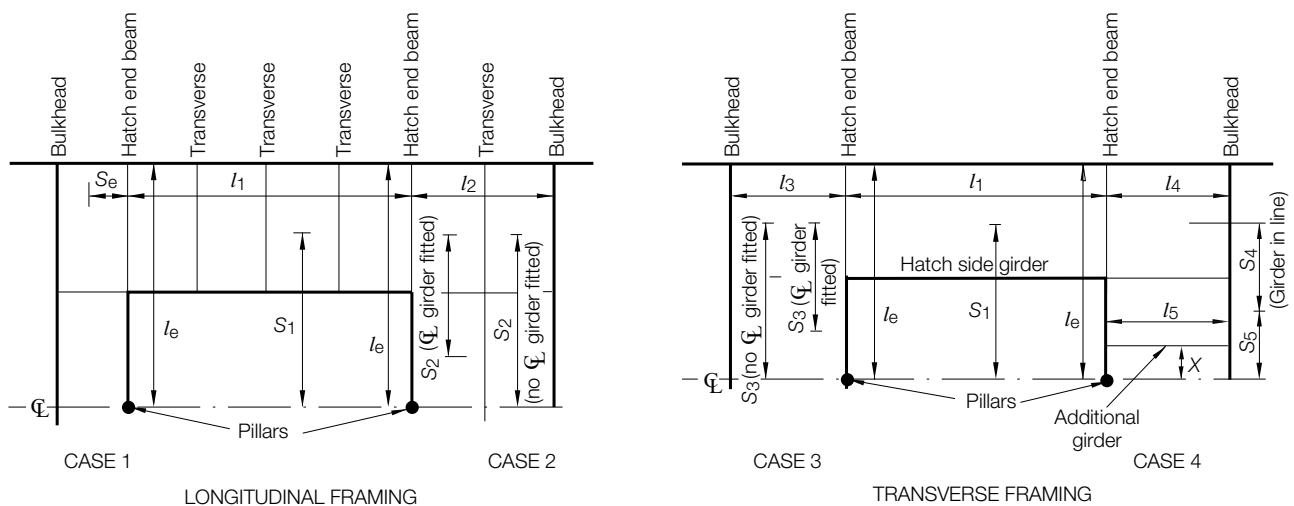
Figure 1.4.1 Hatch end beam arrangements
