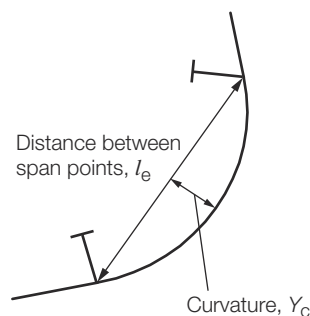
Figure 2.5.1 Distance between span support points and curvature
