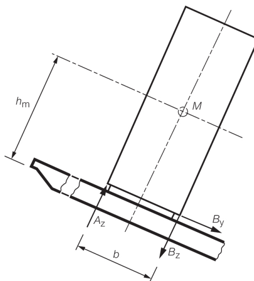
Figure 8.11.1 Forces due to container loads
