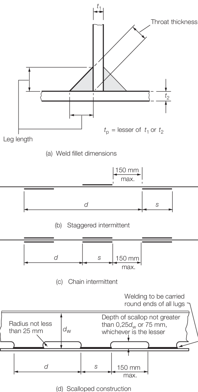
Figure 10.2.1 Weld dimensions and types
