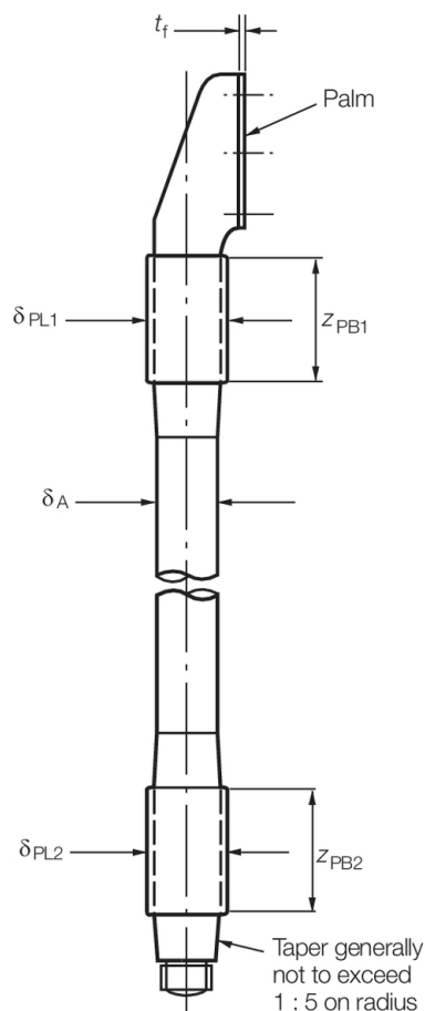
Figure 6.7.3 Rudder axle
