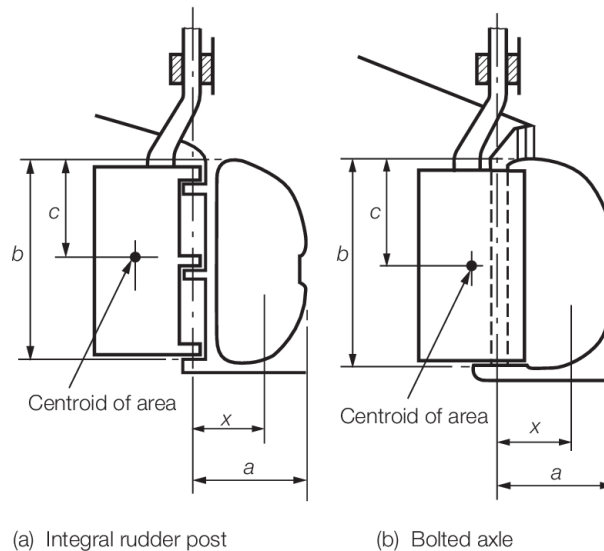
Figure 6.7.6 Solepieces
