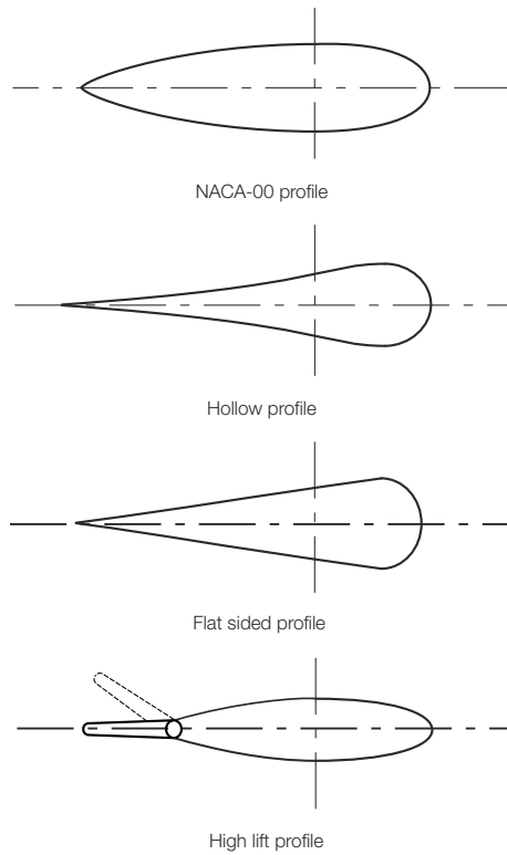
Figure 13.2.1 Rudder profiles
