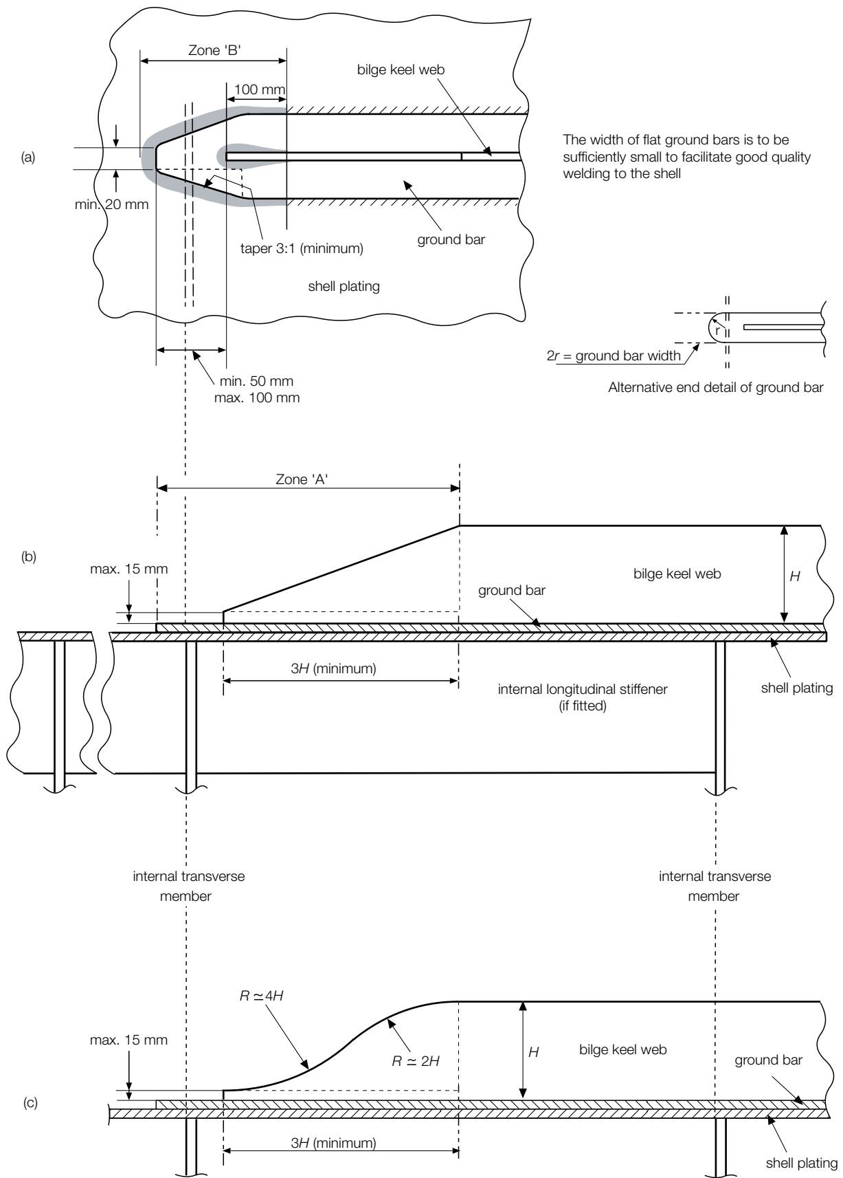
Figure 10.5.5 Bilge keel end design
