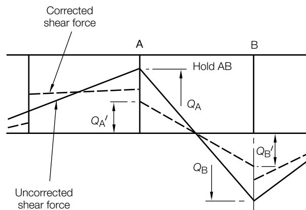
Figure 4.6.2 Shear force correction
