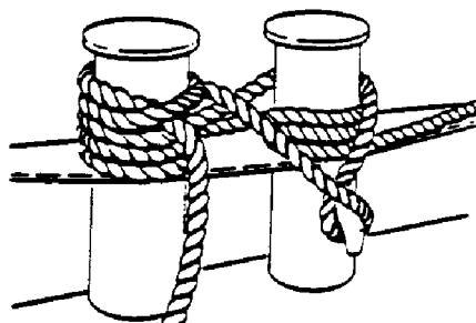
Figure 613-2-31. Correct Method of Making a Side-Tow Hitch
