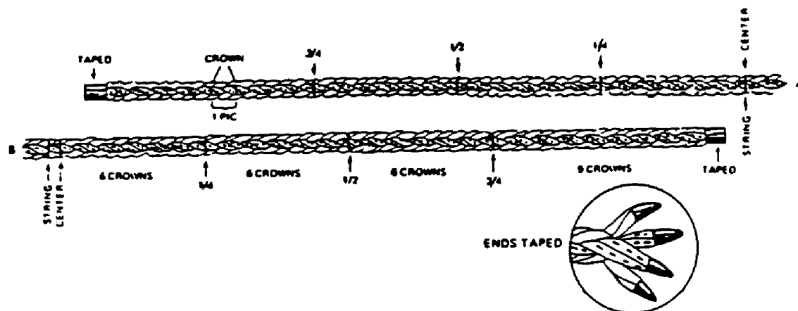
Figure 613-2-16. Preparing Plaited Rope for Long Splice
