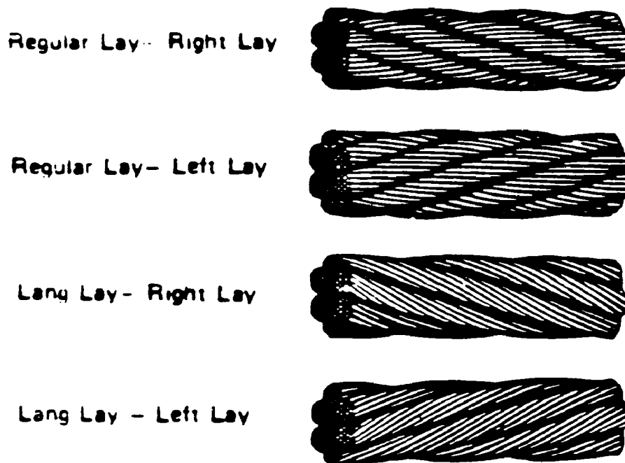
Figure 613-1-3. Wire Rope Lays
