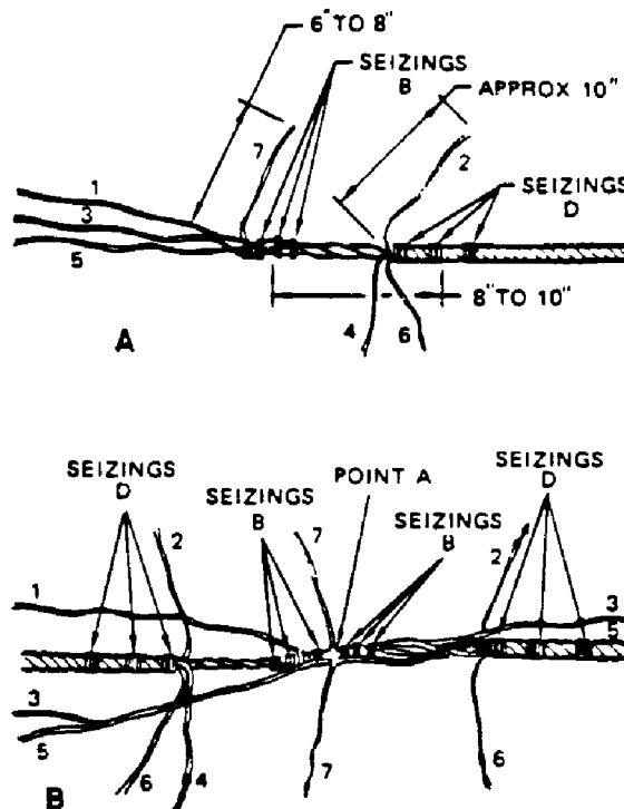
Figure 613-1-36. Butting IWRC Splice
