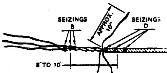
Figure 613-1-24. Seizing Long Splice
