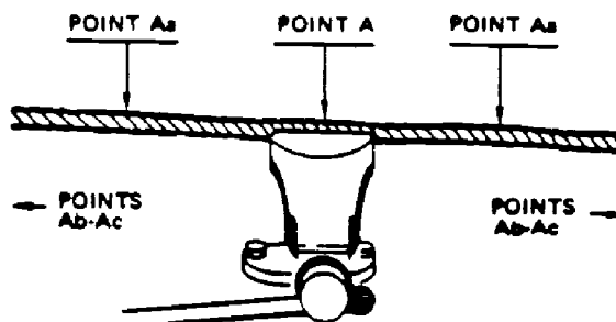
Figure 613-1-40. Finishing IWRC Splice
