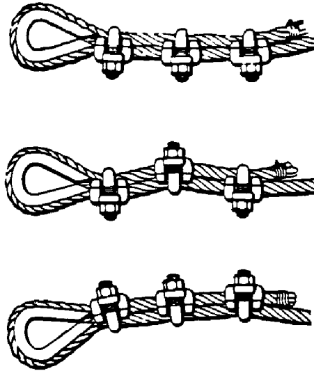
Figure 613-1-23. Clip Attachments
