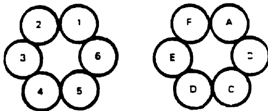
Figure 613-1-25. Strand Identification
