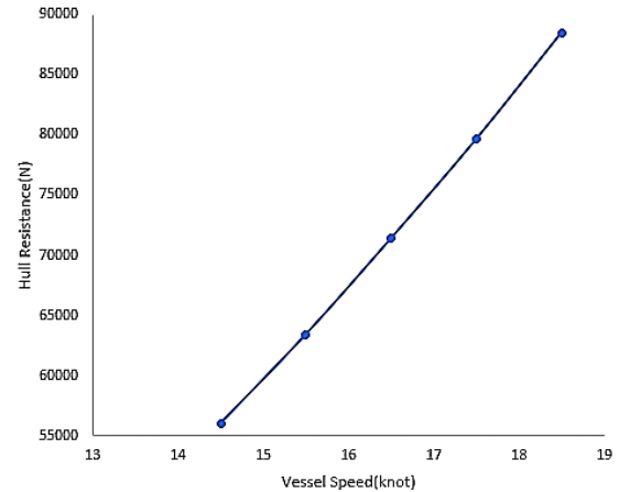
Fig. 5: Total Resistance vs Vessel Speed for Hybrid Propulsion System
