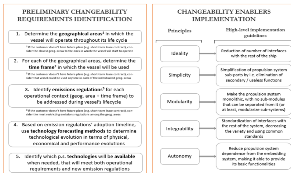
Figure 1 - An approach for maritime propulsion system changeability
