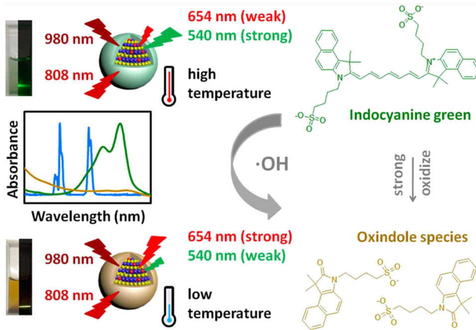
FIGURE 4 Design of the UCNP-ICG, the FRET process, and the response mechanism for \cdot\text{OH} detection Source: Reprinted with permission from American Chemical Society. 105
