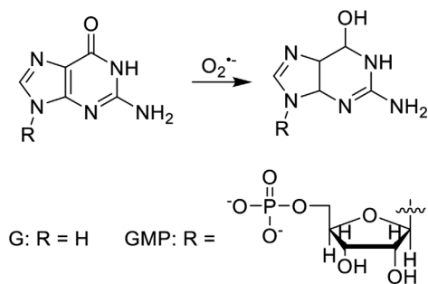
SCHEME 3 Response mechanism of G and GMP with \text{O}_2^{\bullet -}
