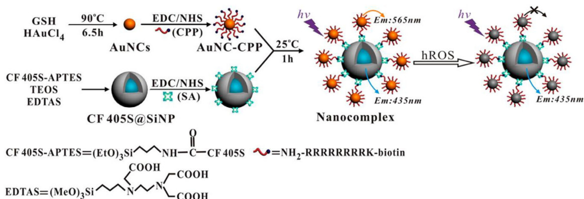
FIGURE 3 Preparation of the AuNC-coated CF405S@SiNP and its response mechanism for •OH detection Source: Reprinted with permission from American Chemical Society. 86
