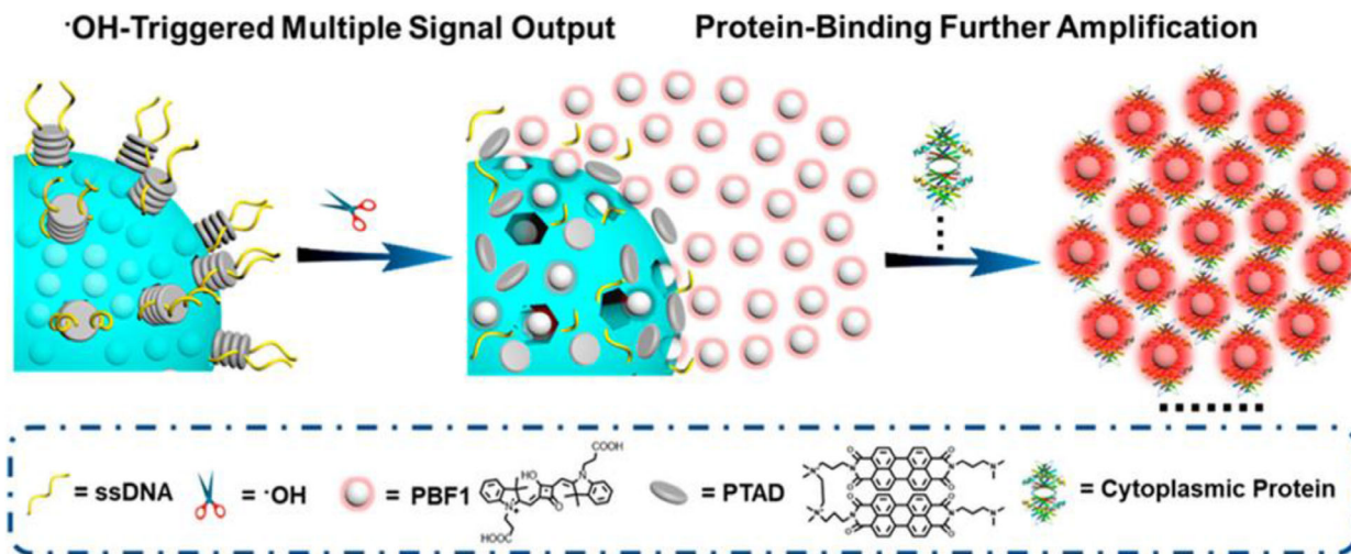
FIGURE 2 Response mechanism of cytoplasmic protein binding based CPFA nanoprobe for •OH and its two-stage amplification process Source: Reprinted with permission from American Chemical Society
