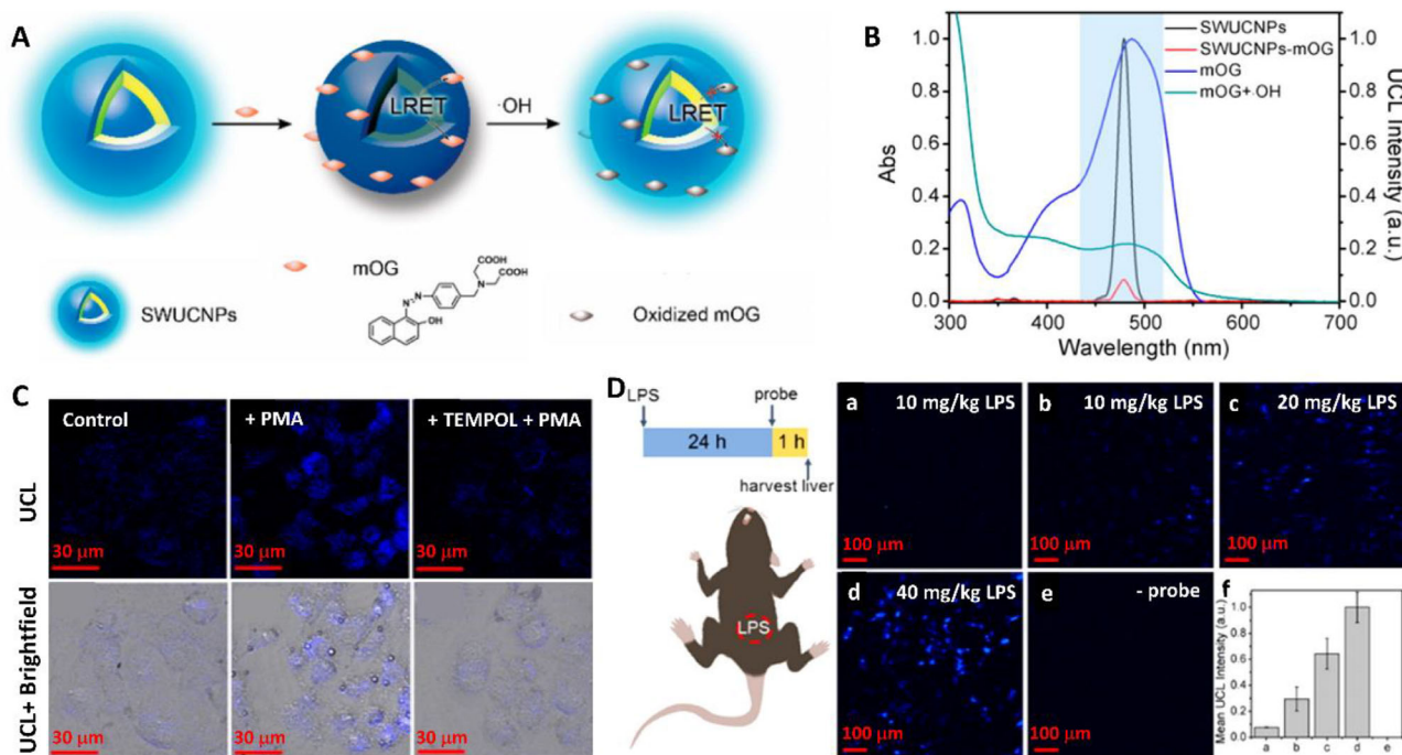
FIGURE 5 mOG-SWUCNPs nanoprobe for \bullet OH detection and UCL imaging
