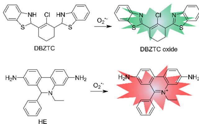
SCHEME 4 Chemical structures of DBZTC and HE and their response mechanisms with \text{O}_2^{\bullet -}
