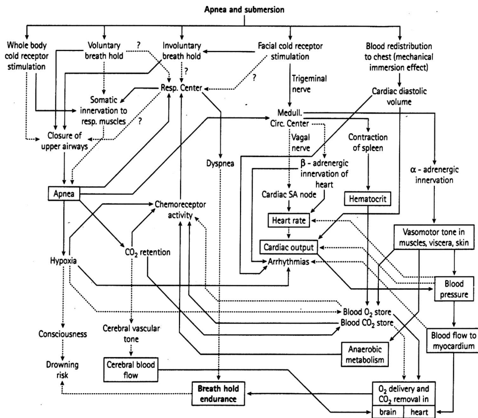
Fig. 2. Schematic of the, often mutually opposing, physiologic reactions to submersed breath-holding. Solid line arrows: at head of arrow, positive influence, i.e., change in 1 direction at tail of arrow promotes change in the same direction; dotted line arrow: negative influence, i.e., change in 1 direction at tail of arrow promotes change in opposite direction at head of arrow. The net effects, known as the diving response, are expressed in the diagram, which is framed. The major components of the diving response are apnea; vasoconstriction in muscles, viscera, and skin; blood pressure increase; bradycardia; lowered cardiac output; elevated brain and myocardial blood flow; increased hematocrit; increased anaerobic metabolism; and preserved O 2 delivery and CO 2 removal in the brain and heart. These changes enhance breath-hold endurance. SA, sinoatrial; Medull., medullary; Circ., circulatory. [Reproduced by permission from Ferrigno and Lundgren (29).]
