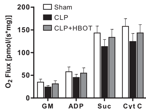
Fig. 3. Hyperbaric oxygen therapy (HBOT) did not impact mitochondrial function after cecal ligation and puncture (CLP). Liver tissues from male CD-1 mice subjected to sham operation ( n = 8 ), CLP + HBOT (2.4 atm. for 1 h at 1 h post-CLP, n = 7 ), or CLP ( n = 7 ) were collected 3 h post-CLP and immediately used to measure oxygen flux under saturating conditions of the following substrates: glutamate and malate (GM) to measure complex I respiration, ADP to measure state III respiration, complex II substrate succinate (Suc) to measure complex I, and complex II respiration combined and cytochrome c (Cyt c ) as a quality control to ensure mitochondrial outer membrane integrity. Oxygen flux is expressed as \text{pmol}\cdot\text{s}^{-1}\cdot\text{mg}^{-1} protein. Values are means \pm SE. Statistical analysis for the comparison between groups was performed by 2-way ANOVA followed by the Tukey's multiple-comparison test. No statistical significance was found.
