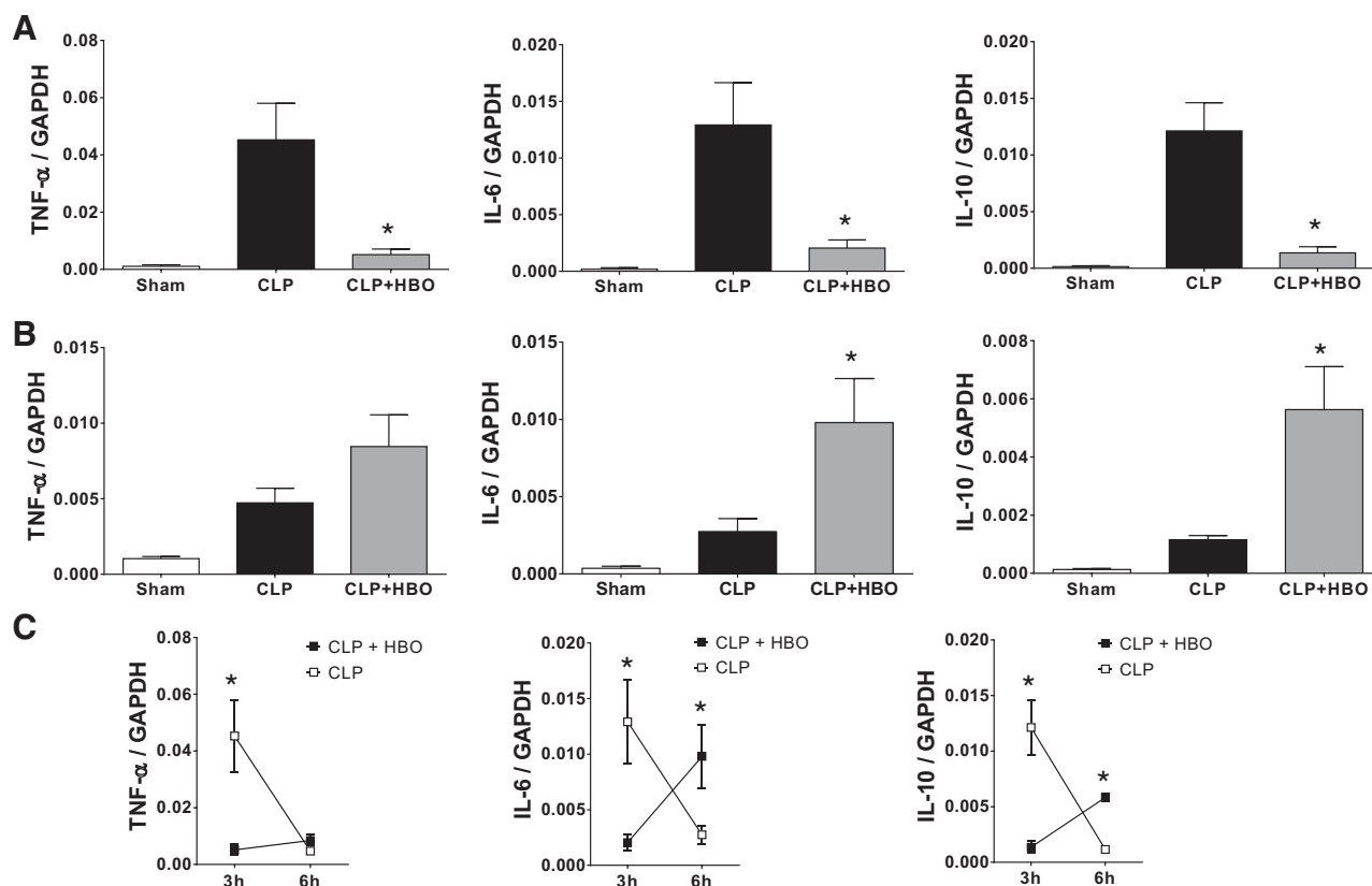
Fig. 4. Inflammatory cytokine expression was altered in mice that underwent hyperbaric oxygen therapy (HBOT) and to cecal ligation and puncture (CLP). Male CD-1 mice (8 wk old) were subjected to CLP ( n = 5 ), CLP + HBOT (2.4 atm, for 1 h at 1 h post-CLP; n = 5 ), or sham operation ( n = 4 ), and liver tissues were collected at 3 or 6 h post-CLP. A and B : cytokine mRNA levels (TNF \alpha , IL-6, and IL-10) were measured by quantitative real-time PCR (qPCR) in the liver samples obtained at 3 ( A ) or 6 h ( B ) post-CLP. C : kinetic expression of TNF \alpha , IL-6, and IL-10 is depicted. Values are means \pm SE, and statistical analysis for the comparison between groups was performed by 1-way ANOVA followed by Tukey's multiple-comparison test ( A and B ) or 2-way ANOVA followed by the Bonferroni's multiple-comparison test ( C ). * P < 0.05 , comparing CLP and CLP + HBO groups.
