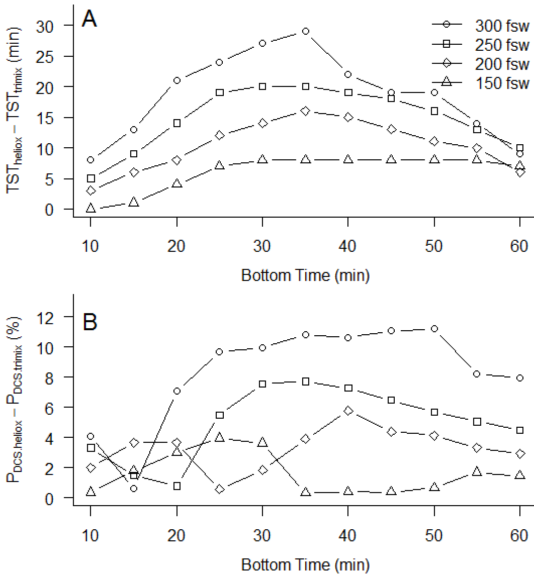
Figure 1. Panel A shows the difference in total decompression stop times (TST) in minutes between trimix and heliox MK 16 MOD 1 decompression schedules calculated with LEM-he8n25 for a target P_{DCS} of 2.3%. Panel B shows the increase in LEM-he8n25-estimated P_{DCS} for MK 16 MOD 1 heliox dives conducted on trimix decompression schedules calculated for a target P_{DCS} of 2.3%. In Panel B, the schedules included a 30-minute period of breathing 0.70 atm PO_2 heliox or trimix on the surface before descent. In both Panels A and B, the decompression schedules were calculated for inspired gas in which the inert gas component was either all helium (heliox) or equal parts helium and nitrogen (trimix). The decompression schedules in Panels A and B were calculated with the following conventions used to calculate the MK 16 MOD 1 He- O_2 decompression schedules in the U.S. Navy Diving Manual: a descent rate of 60 fsw/min; an ascent rate to and from stops of 30 fsw/min; a 20 fsw last stop depth; and an inspired gas with constant oxygen partial pressure ( PO_2 ) of 0.70 atm from the surface until descent past 32 fsw, then a constant PO_2 of 1.3 atm, and a PO_2 of 0.70 atm on ascent shallower than 12 fsw.
