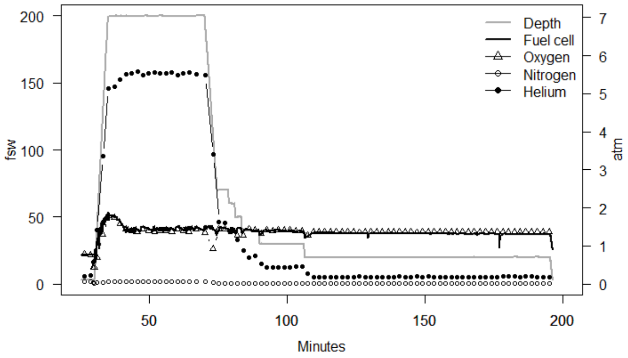
Figure 4. UBA gas composition during a trimix dive (top) and heliox dive (bottom). The depth in fsw gauge is indicated on the left axis and gas partial pressures in atmospheres are indicated on the right axis. The traces with symbols indicate oxygen, nitrogen and helium partial pressures calculated from the ambient pressure in the wet pot and the fractions of these gases analyzed with mass spectrometer. The solid black trace (Fuel cell) is oxygen partial pressure calculated from the output of the K-1D micro-fuel cell oxygen sensor.
