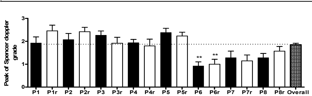
Fig. 1b: Doppler Grade Variations (SS) after each dive profile. The comparison of means has been done computing the peak Doppler scores for each individual after each dive profile according to the Expanded Spencer Scale (ESS) and Spencer Scale (SS). The means have been compared using parametric tests when possible after KS normality testing (ANOVA with Neuman-Keuls post tests) and Kruskal-Wallis and Dunn’s post test when the normality testing does not allow parametric evaluation. By accepting a ESS score of 1.5 and an SS score of 2 as “safe”, it can be seen that the deep stop appears “safer” using both ESS and SS scales, while repetitive profiles 1,2,3 and 5 are “unsafe”.
