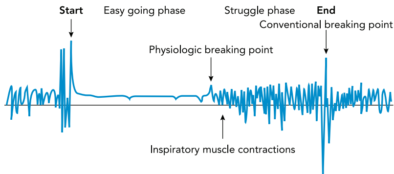
FIGURE 2. Human thoracic movements measured by electromyography (EMG) during maximal breath-holding in an untrained, non-immersed subject. “Easy going phase” and “struggle phase” are distinguished by the absence or presence of respiratory muscle activity that must be suppressed during breath-holding. Figure is from Ref. 72 and used with permission from Saunders.
