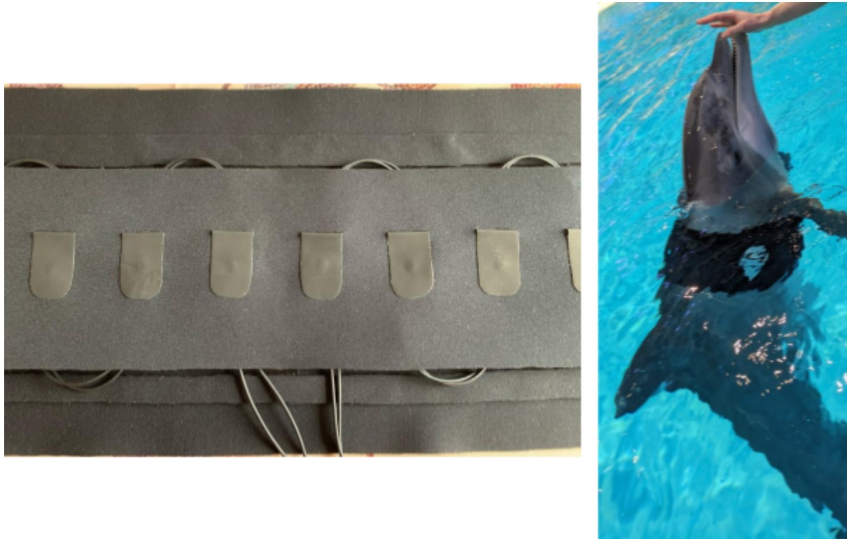
Figure 5: Modified EIT belt and its use on a dolphin. Left: The EIT electrodes are made of conductive carbon film with a rear snap connector to the cables. All other parts are neoprene, including an outer layer to prevent current leakage. Right: The belt placed on a dolphin during habituation.
