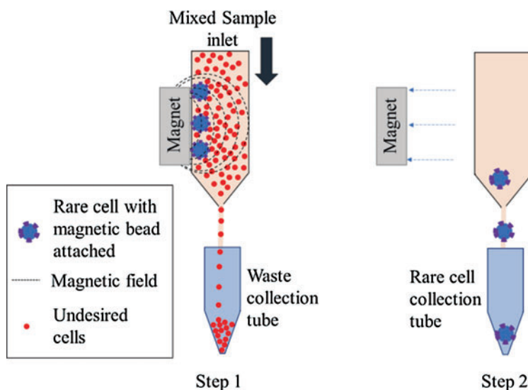
Fig. 4 Magnetically activated cell sorting (MACS) is achieved by attaching antibody-coated magnetic nanometer-sized beads to the cells of interest
