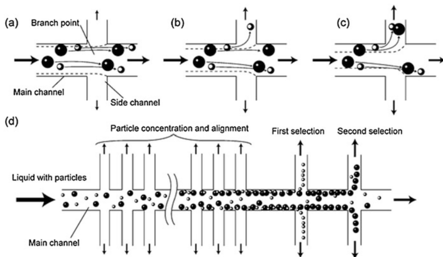
Fig. 9 Schematic diagram of hydrodynamic cell separation device. (Reproduced by permission of the Royal Society of Chemistry Yamada and Seki 2005)
