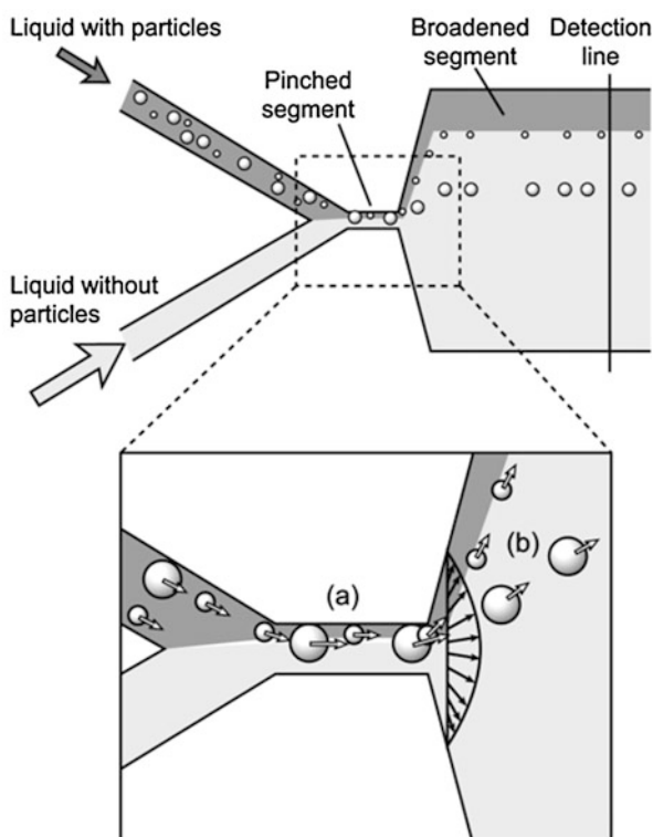
Fig. 8 Pinched flow fractionation. A buffer stream focuses the particle stream against the wall in the pinched channel. Due to the difference in their sizes, larger and smaller particles follow different streamlines when they are focused. When channel widens, smaller cells continue to flow near to the wall and larger cells shift near the center. As the cells of different sizes follow different streamlines in the laminar flow, they can be collected in different outlets. (Reproduced by permission of the ACS publications Yamada et al. 2004)
