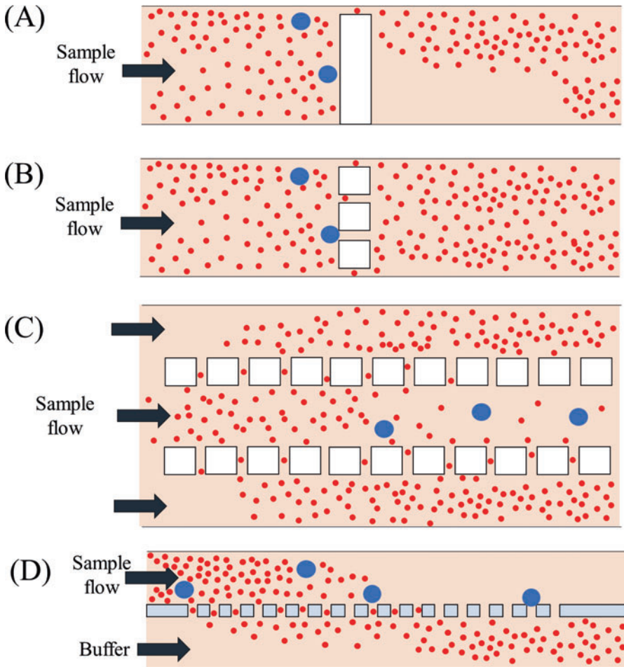
Fig. 6 Schematic diagram explaining different filter-based cell sorting methods. (a) Weir filter (side view). (b) Dead-end pillar filter (top view). (c) Cross-flow filter (top view). (d) Membrane filter (side view)
