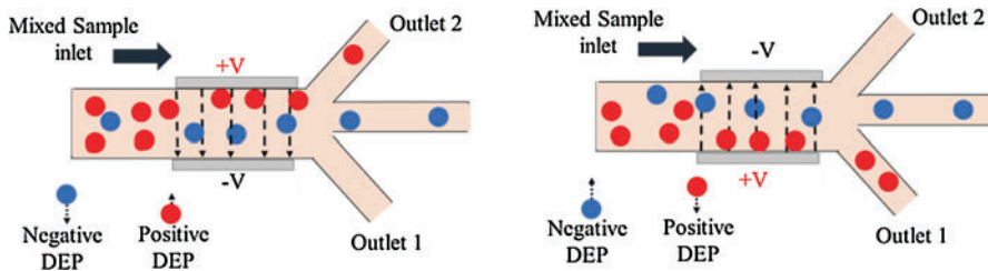
Fig. 10 Schematic diagram explaining dielectrophoresis (DEP). In positive DEP, particles move toward the higher electric field. In negative DEP, the particles move toward the electric field minima
