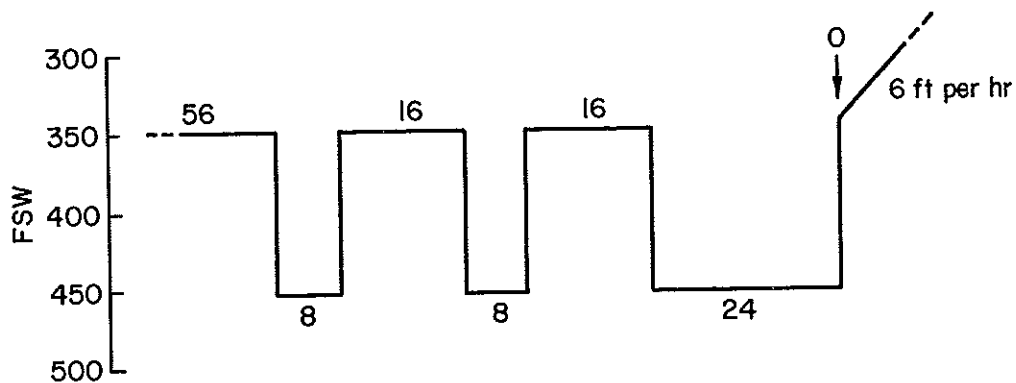
Fig. 3. Profiles of excursions, 106 ft from 456 to 350 fsw, and initial hours of saturation decompression. Duration at each depth is indicated in hours on the profile.
