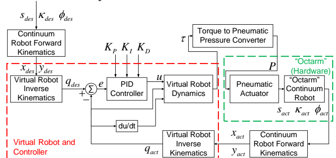
Fig. 2. Block Diagram for Continuum robot control based on virtual robot models.
