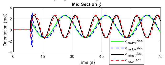
Fig. 13. Two section experiment 2 (OctArm tip and mid sections) — Desired and actual mid-section orientation under slow and fast speed rotations.
