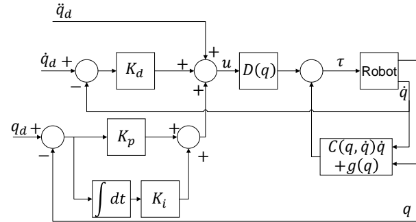
Fig. 5. Block diagram for computed-torque controller designed for virtual RRRR (one-section) and RRRRRR (two-section) robot.
