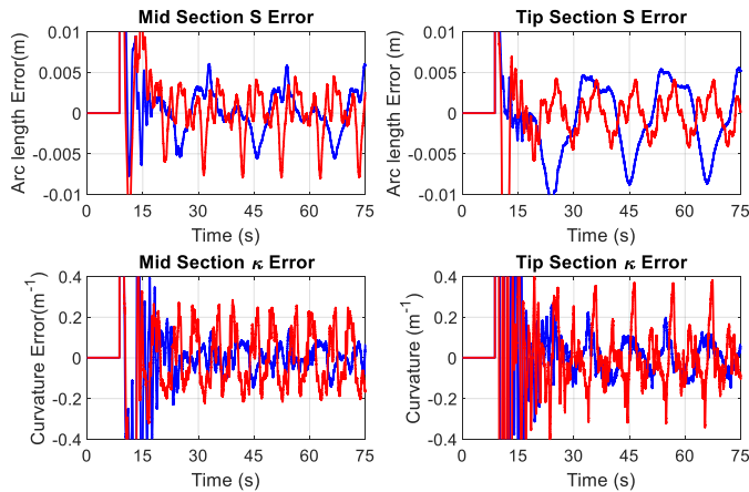
Fig. 15. Two section experiment 2 (OctArm tip and midsection) — Arc length s , and curvature \kappa error on OctArm in configuration space (slow rotation in blue line, and fast rotation in red line)
