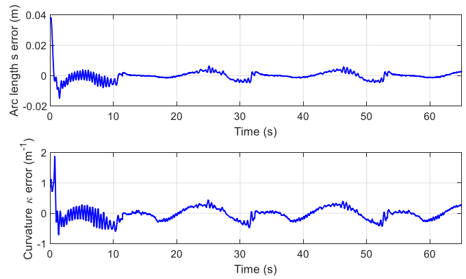
Fig. 9. One section experiment (OctArm tip section) — Arc length s , and curvature \kappa error on OctArm in configuration space
