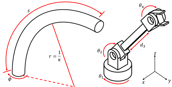
Fig. 3. Continuum robot section (left), is modeled based on virtual RRPR discrete-jointed robot (right).
