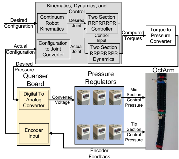
Fig. 7. Experimental control loop block diagram for two section OctArm virtual 8-DoF RRRRRRPR discrete-jointed model dynamics control.
