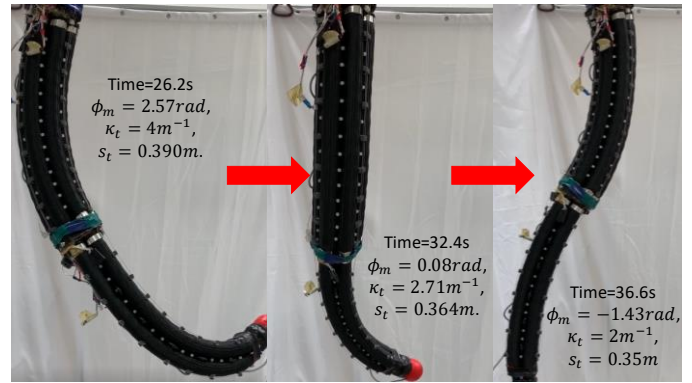
Fig. 16. Two section experiment 3: Mid-section rotates from 2.57rad to -1.43rad while the tip section curvature and arc length follows a sinusoidal path. The tip section at 26.2s is more curled than the tip section at 36.6s.
