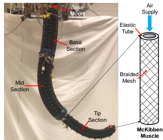
Fig. 1. Dynamically controlled OctArm, a pneumatically actuated continuum manipulator with three sections, following a desired configuration trajectory.
