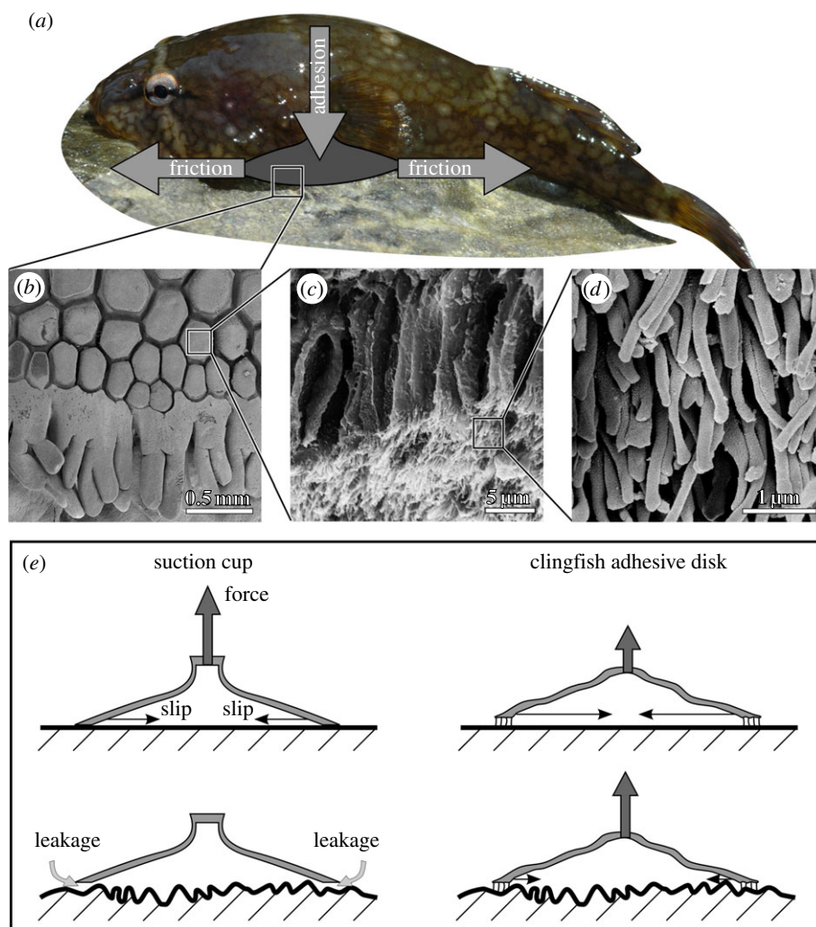
Figure 2. Effectiveness of the clingfish adhesive disc. (a) A clingfish adhering to a rock surface. Two types of forces act on the clingfish adhesive disc. (i) Adhesion acts normal to the surface and holds the fish to the rock; and (ii) friction acts parallel to the surface and prevents sliding of the disc along the substrate. (b) SEM of the ventral surface of the adhesive disc showing the tiled papillae covered in mucus and the fimbriated edge of the adhesive disc. Papillae occur at the edges of the suction disc and other points of surface contact. (c) SEM of a papilla, consisting of multiple rods subdivided apically into fine filaments. (d) SEM of the filaments on the tips of the rod-like structures. (e) Schematic cross sections through a manufactured suction cup and a clingfish adhesive disc. Pulling on a suction cup causes its sides to slip inward. The filaments on the disc of clingfish cause higher friction and prevent slipping on rough surfaces. The flexibility of the disc and its filaments allow for sealing on rough surfaces, whereas the stiff manufactured suction cups fail owing to leakage.
