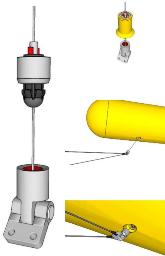
Figure 11 Orbital O2 mooring connector
