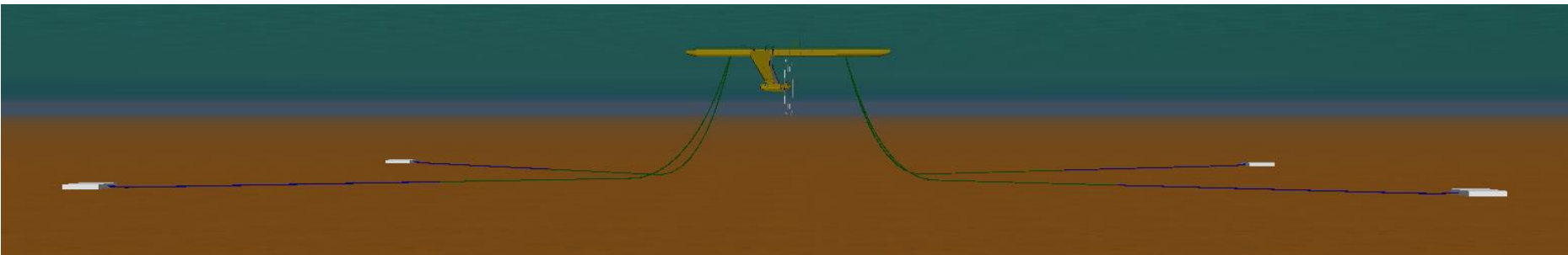
Figure 6 Orbital O2 mooring system at slack tide (green lines are 95mm Studlink chain, blue lines are 115mm studlink)
