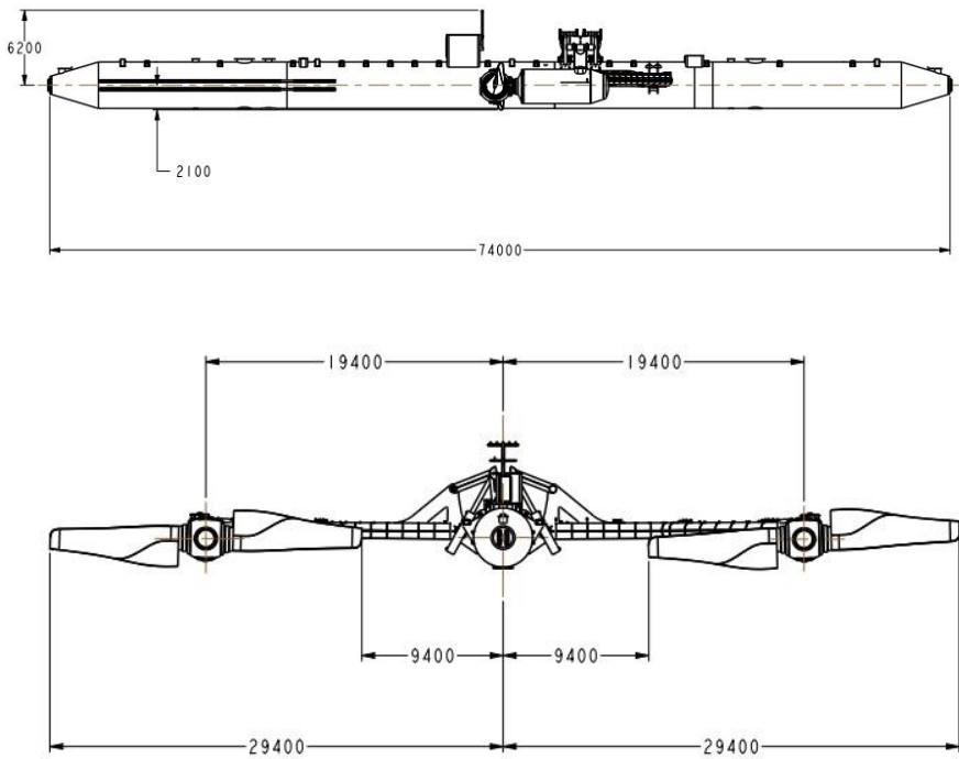
Figure 2 Orbital O2 in transport mode
