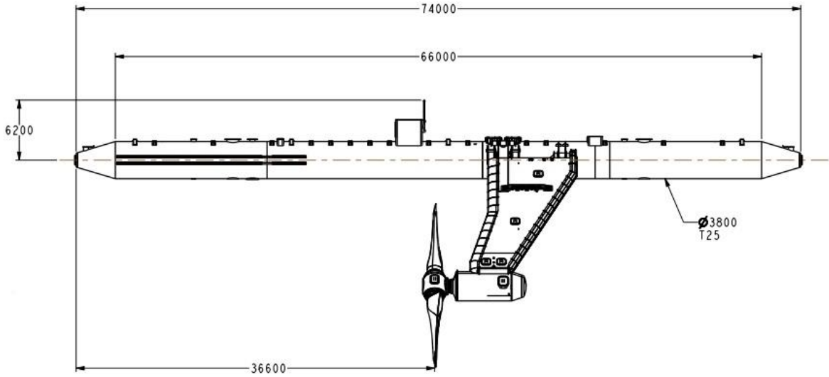
Figure 2 Orbital O2 in transport mode
