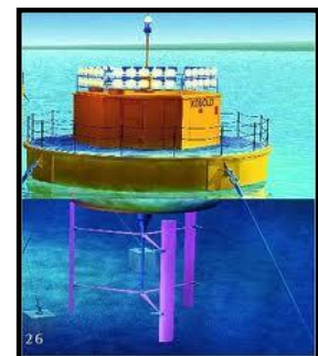
Fig. 4.16. Kobold turbine [XV]
