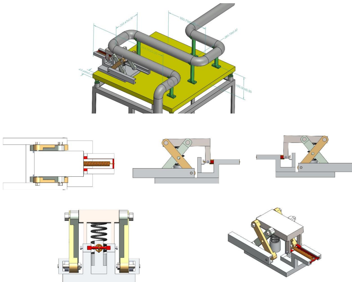
Figure 7: Complete CAD model
