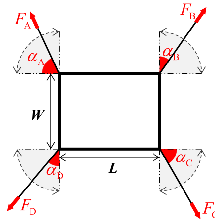
Fig. 2. Force diagram of the offshore platform.
