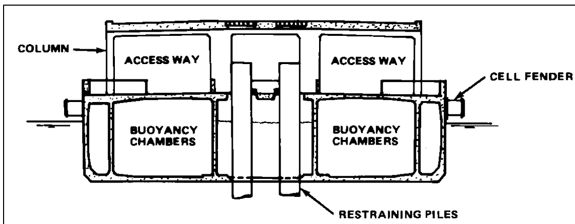
Figure 2-4 Floating Pier Design Concept
