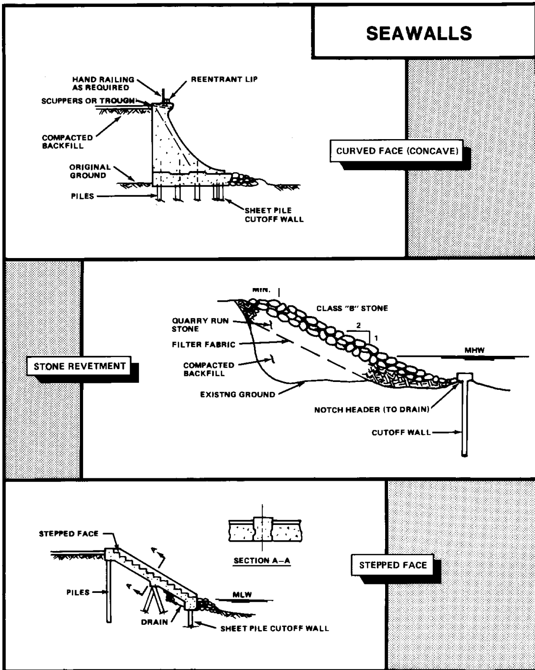
Figure 2-6 Seawall Configurations
