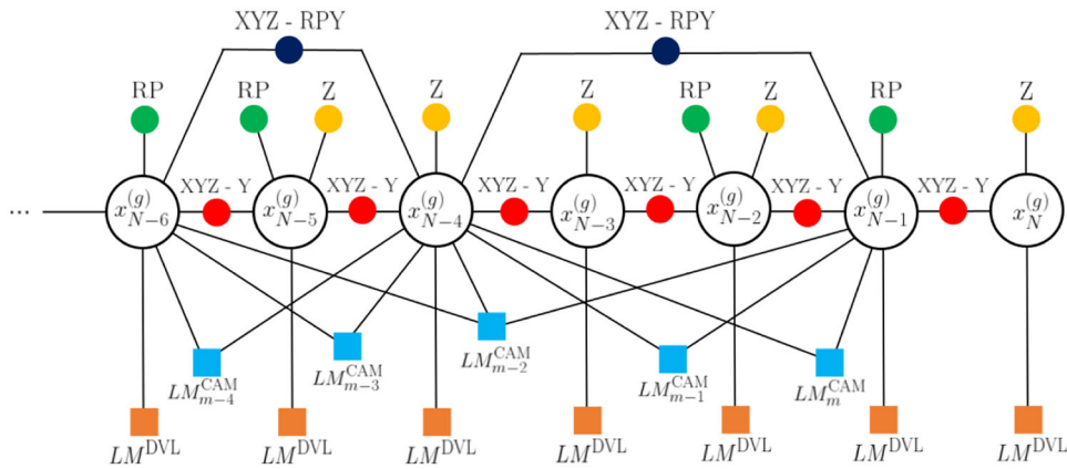
FIGURE 3 Last nodes of the factor graph g constrained with vision-based landmarks and all the onboard sensors. CAM, camera; DVL, Doppler Velocity Log.
