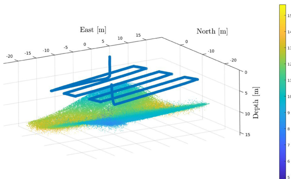
FIGURE 16 Filtered point cloud and estimated trajectory traveled by the simulated vehicle. The values reported in the color map are in meters.
