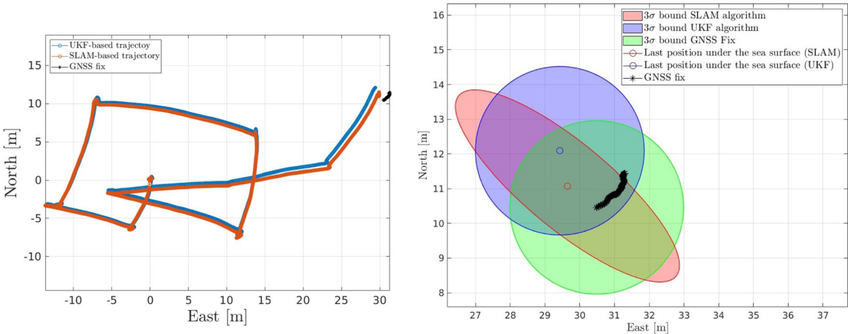
FIGURE 13 On the left, comparison between the trajectories estimated with the SLAM algorithm and the UKF algorithm during the mission accomplished in Stromboli Island, Messina (Italy). A ground truth, when the vehicle was under the sea surface, is not available, but the first GNSS fix when the vehicle resurfaces can be employed as a reference to evaluate the resurfacing error. On the right, the 3\sigma bound of the last positions under the sea surface is estimated with the SLAM and UKF algorithms and the first GNSS fix measurement with its accuracy 3\sigma bound. The trajectory estimated through the SLAM algorithm has been computed before the outlier rejection, which has been employed only for the seabed 3D reconstruction. 3D, three-dimensional; GNSS, Global Navigation Satellite System; SLAM, Simultaneous Localization and Mapping; UKF, Unscented Kalman Filter.
