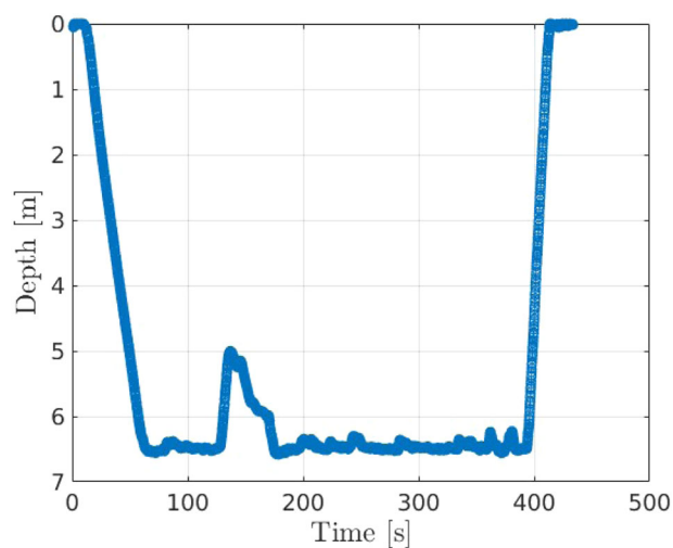
FIGURE 10 FeelHippo AUV depth profile during the mission in Stromboli Island, Messina (Italy). AUV, Autonomous Underwater Vehicle.
