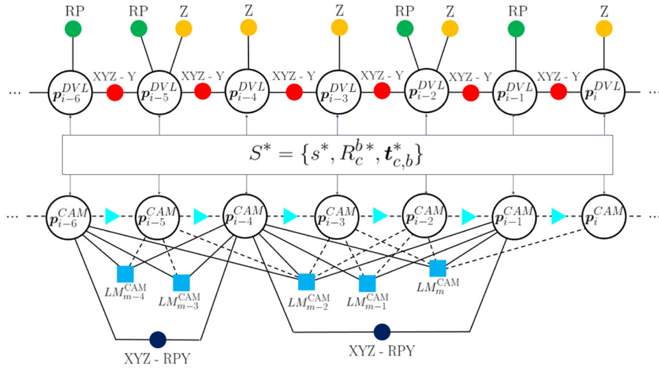
FIGURE 2 Comparison of the two-factor graphs (e.g., the DVL-based graph on the top and the camera-based graph on the bottom of the image) employed for the scale factor ambiguity resolution. The dashed lines in the bottom graph are the edges which are not reported in the whole graph. For ease of reading, a one-to-one association between the two graphs is considered. CAM, camera; DVL, Doppler Velocity Log.
