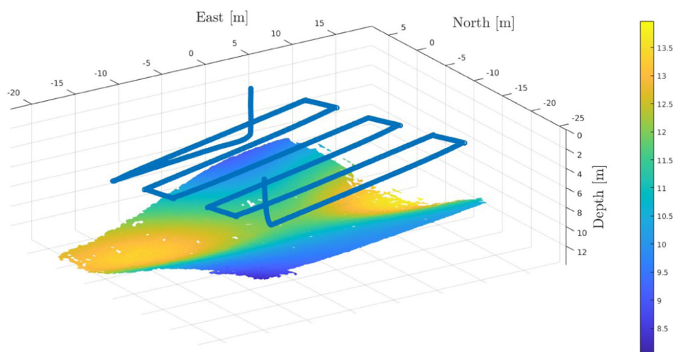
FIGURE 19 Resulting sea bottom three-dimensional mesh reconstruction and estimated trajectory traveled by the simulated vehicle. The values reported in the color map are in meters.
