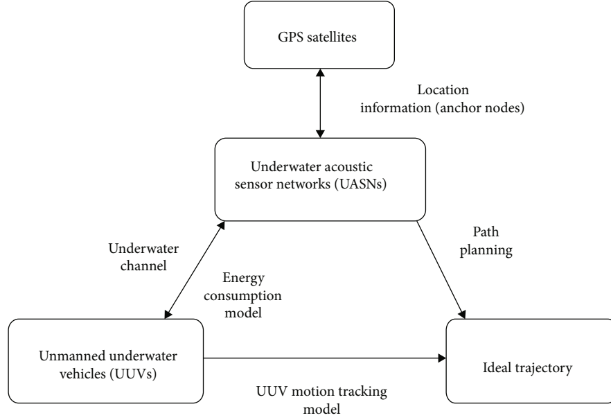
FIGURE 2: Illustration of the UASN, where the UUV receives the message from anchor nodes to position itself for trajectory correction.
