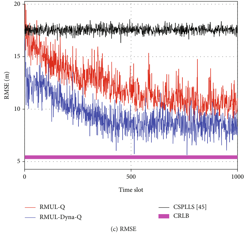
FIGURE 9: Performance in the underwater environment.
