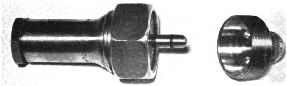
PLATE 71-C.—Diving telephone coupling, male (jack plug housing)—Assembled.
