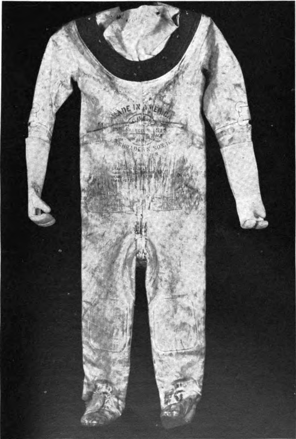
PLATE 22.—Standard diving dress, with gloves attached—Front view.
