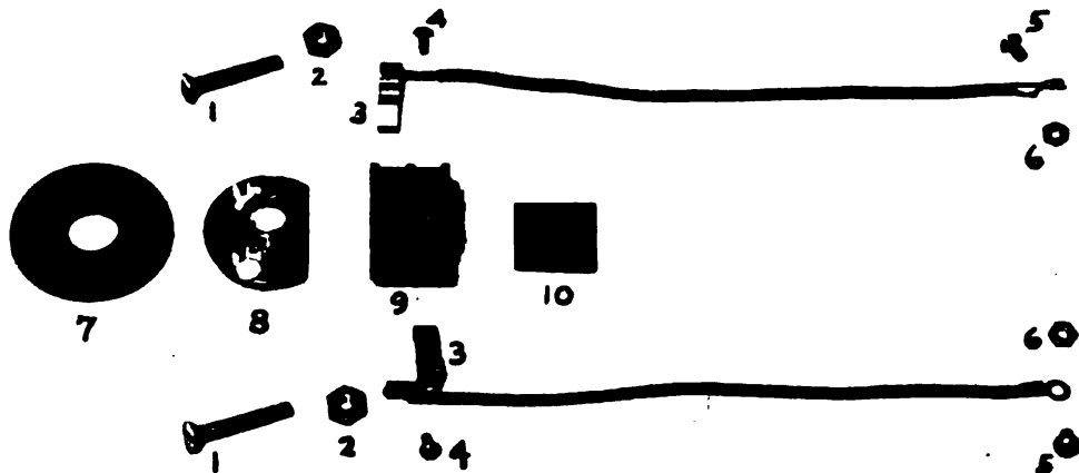
PLATE 71-F.—Diving telephone coupling, for helmet gooseneck (female connection)— Disassembled.
