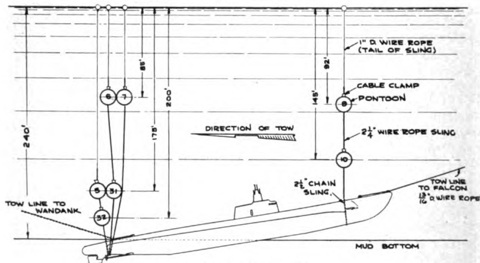
ARRANGEMENT OF PONTOONS LIFT OF 13 JULY, 1939 SCALE \frac{1}{2}'' = 1'-0''
