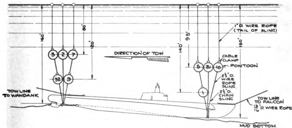
ARRANGEMENT OF PONTOONS LIFT OF 17-AUG, 1939 SCALE: \frac{1}{80}'' = 1'-0''
