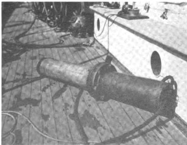
PLATE 5—FIGURE 3.—Sample of flanges fitted under water by student divers.
