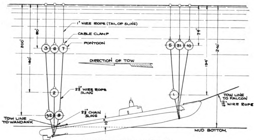
ARRANGEMENT OF PONTOONS LIFT OF 12 AUG. 1939 SCALE: \frac{1}{80}'' = 1'-0''
