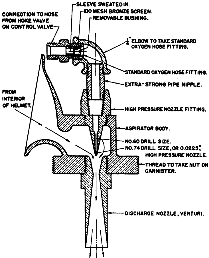
PLATE 97.—Helmet oxygen-helium, cross section of aspirator and discharge nozzle venturi.
