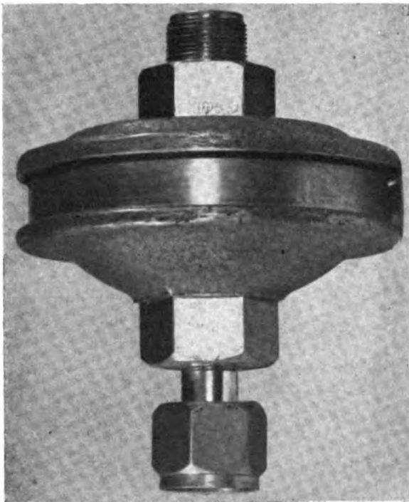
PLATE 63.—Oil separator—Assembled.
