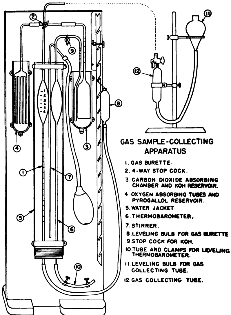
PLATE 91.—Haldane-Henderson gas analysis apparatus.
