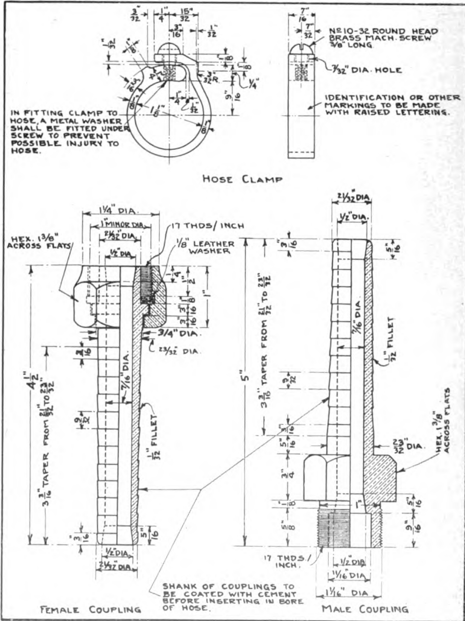
PLATE 30.—Diving air hose couplings and clamps.
