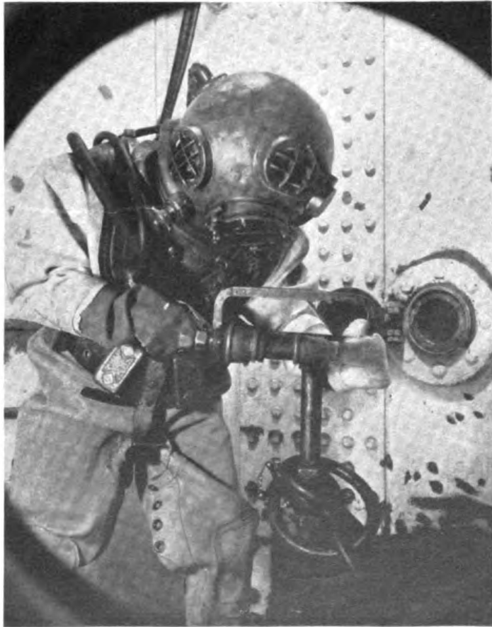
PLATE 2—FIGURE 2.—Diver in water diving tank sawing through a section of steel piping.
