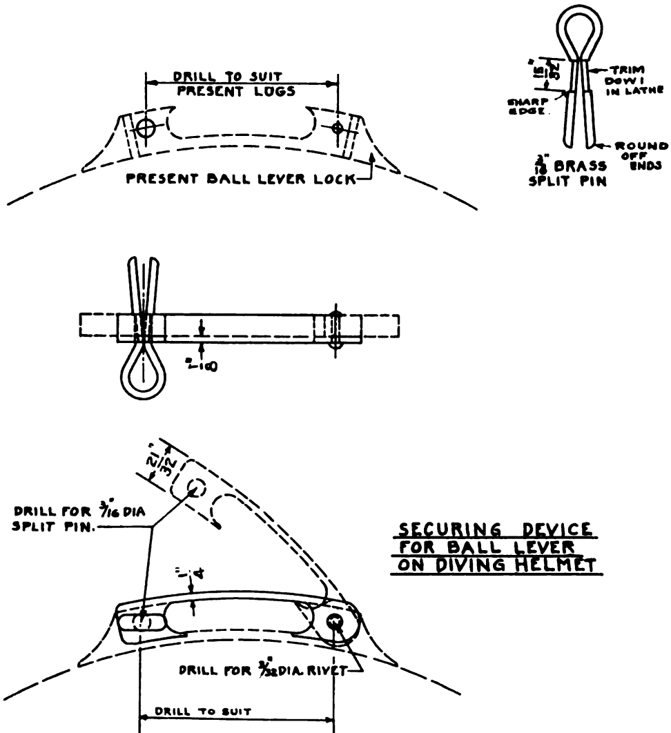
PLATE 25.—Helmet lock.
