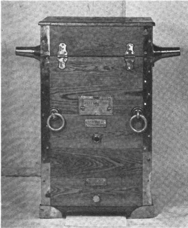
PLATE 56.—Navy standard diving air pump, Mark III, assembled— Back view.
