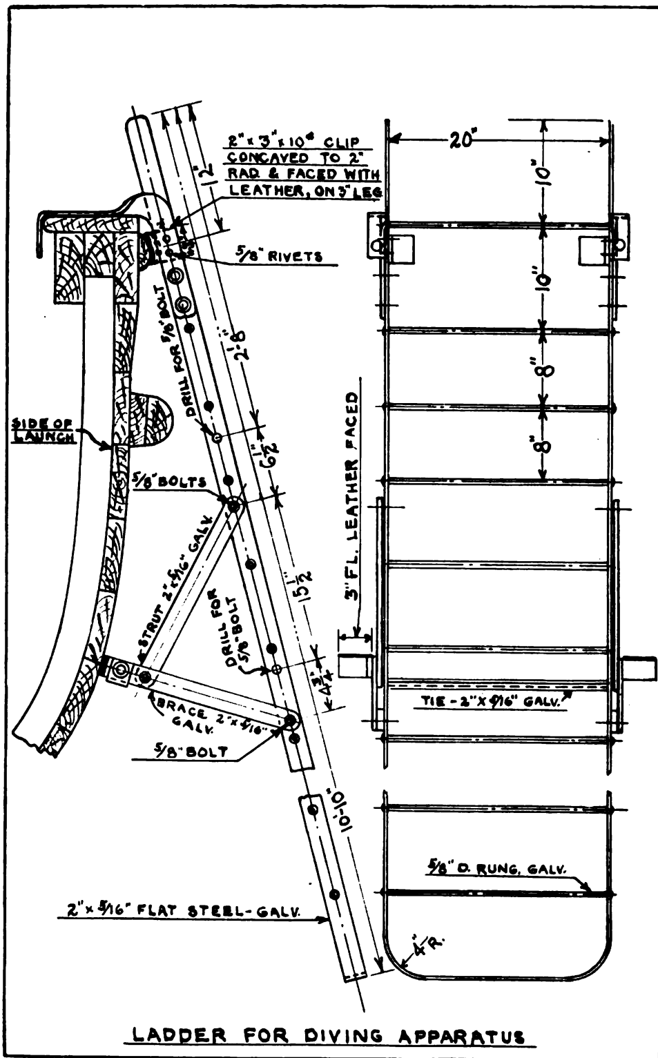
PLATE 34.—Diving ladder.
