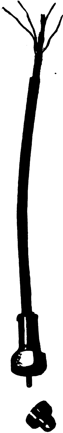
PLATE 14.—Standard rubber-covered combination telephone and life-line cable.
