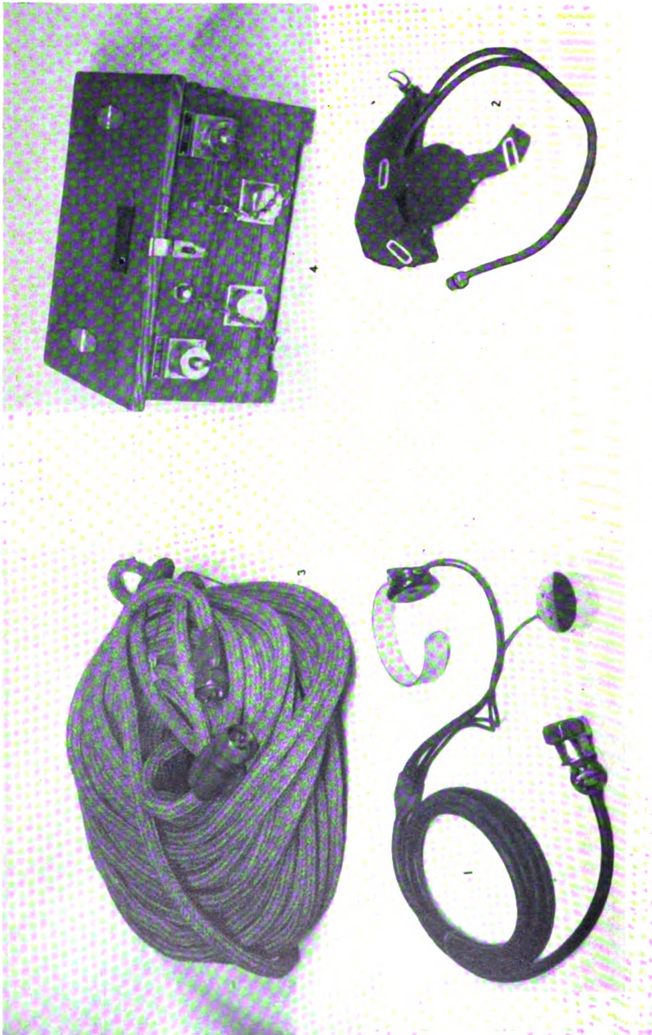
PLATE 72.—Diving telephone, battery type, and sennet-covered combination telephone and life line cable.
