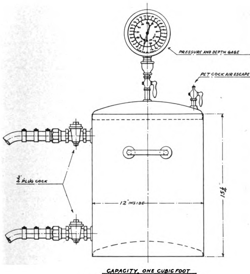
PLATE 74-A.—Tank, test, for diving air system.
