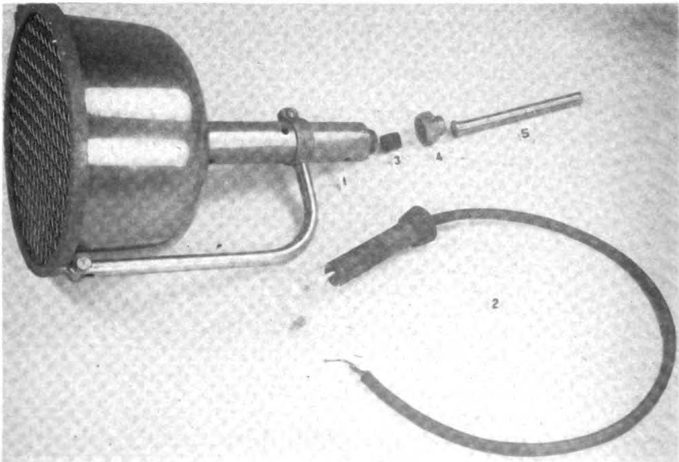
PLATE 51.—Diving light, Westinghouse Lamp Co. type—Disassembled.
