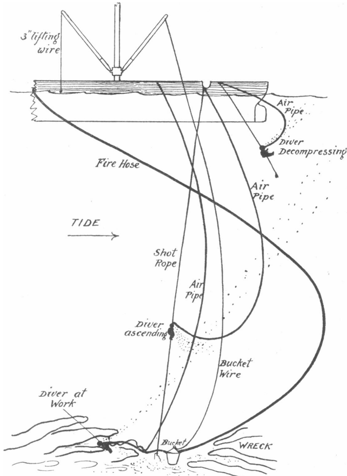
Text-fig. 5. Diagram illustrating the lay in the water of the air pipes, water hose and wire ropes.
