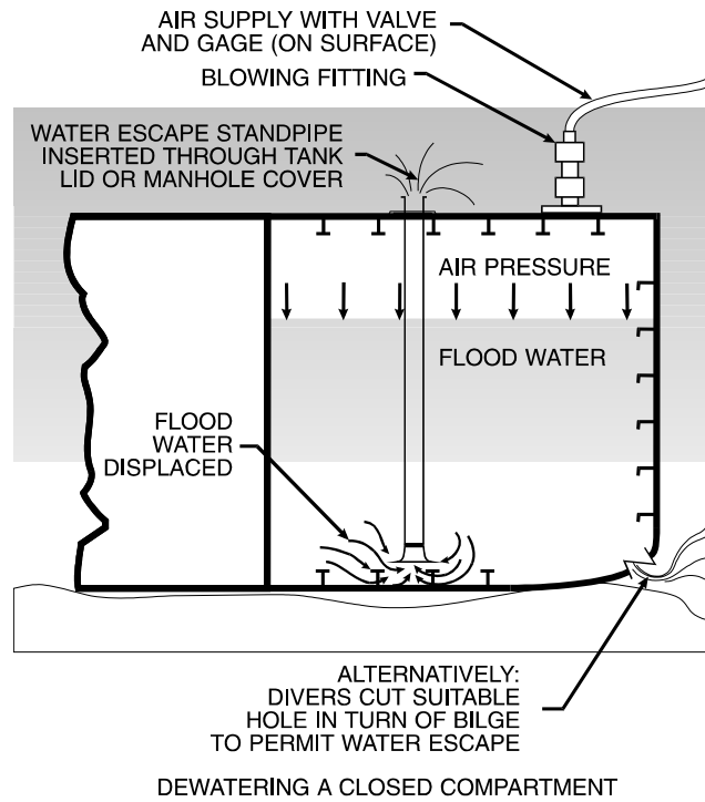
Figure 5-20B. Blowing Techniques.
