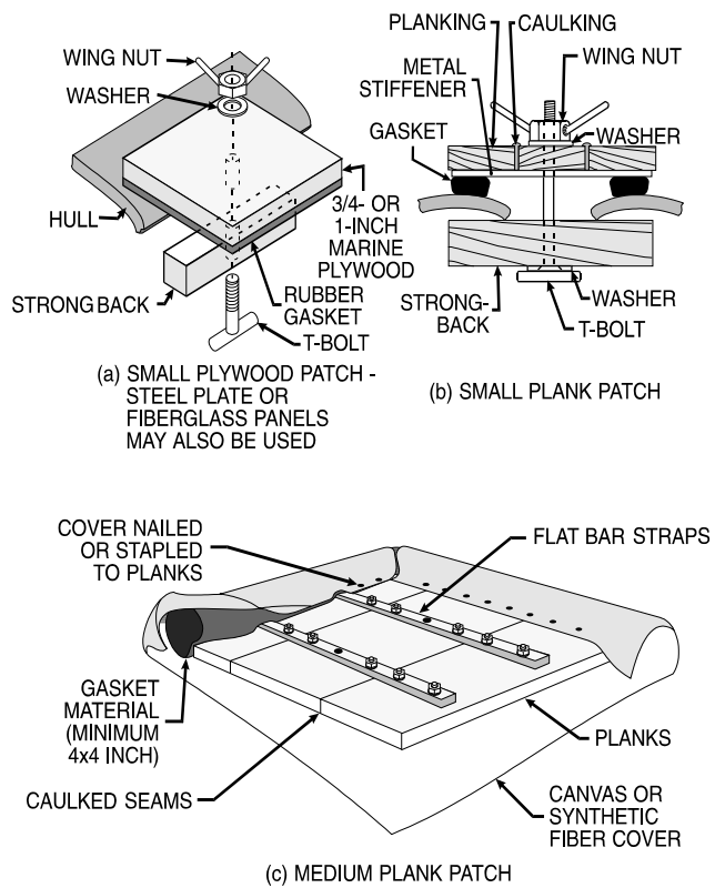
Figure 5-4. Wooden Patch Construction.
