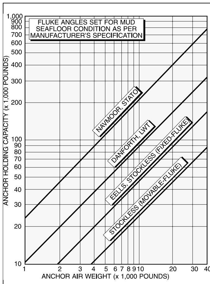
Figure 3-9. Drag Anchor System Holding Capacity in Mud.
