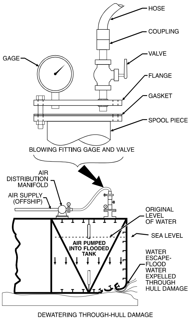
Figure 5-20A. Blowing Techniques.
