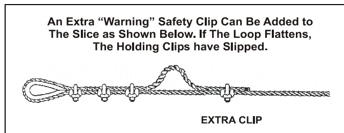
Figure 3-5. Joining Wire Ropes.
