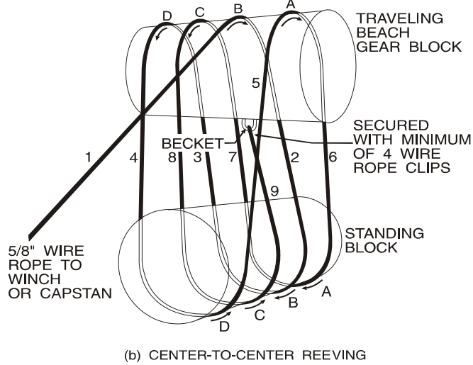
Figure 4-4 Reeving Blocks
