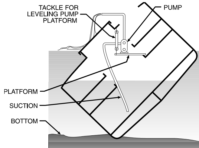
Figure 5-19C. Pumping Arrangements.
