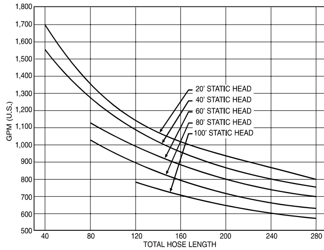
Figure 7-4J. Performance Curve (Water), CCN-150 Pump (4" Hose).
