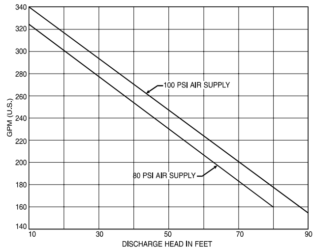
Figure 7-4D. Performance Curve, 2 1/2" Air Submersible Pump.
