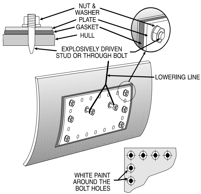
(a) BOLTED STEEL PATCH
