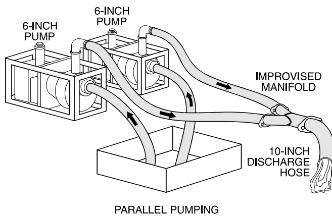
Figure 5-19B. Pumping Arrangements.
