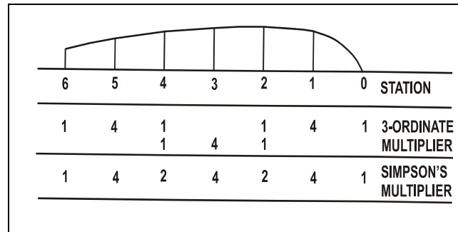
Figure 2-11. Simpson's Multipliers for Long Curve.
