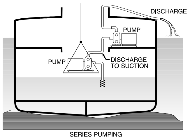
Figure 5-19A. Pumping Arrangements.
