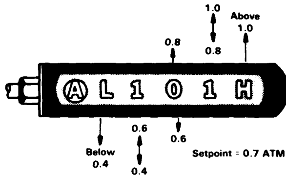
Figure 11-22 Primary display
