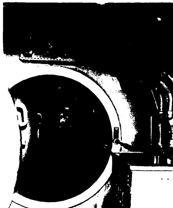
Figure 13-10 DDS MK 2—Deck Decompression Chamber Out Lock Interior
