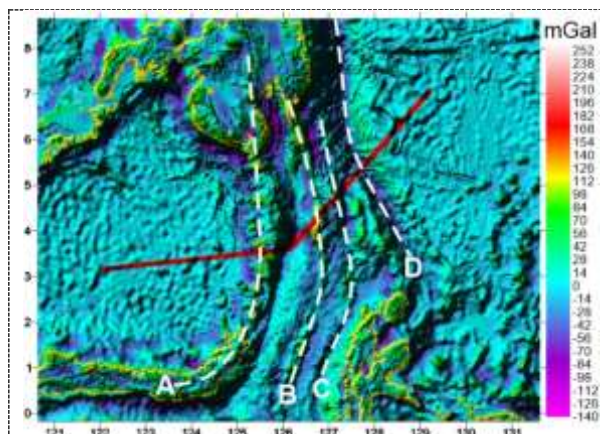
Figure 4. Overlapping residual gravity data in milliGal unit on the bathymetry elevation model from GEBCO, solid lines are the section profile, and dotted lines are the interest line areas.
