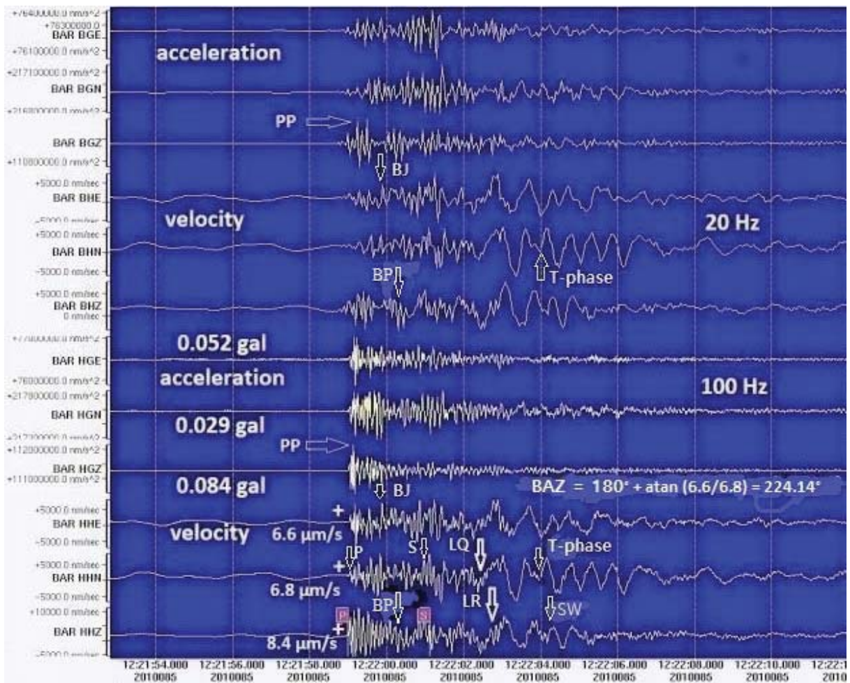
Figure 2: Seismogram and accelerogram showing the velocity ( \mu\text{m/sec} ) and acceleration (g) that were recorded with 20 and 100 SPS (samples per second) for the underwater explosion of ROKS Cheonan at the Baengnyeong Island station (BAR, KMA) in the Yellow Sea of the Korean Peninsula [4,5]. The polarities (+), the arrow marks for bubble pulses (BP), bubble jets (BJ) and P- (P), S- (S), Love (LQ), Rayleigh (LR) [6], Stoneley (SW) [7], T (T-phase) [8] waves, and a back azimuth (BAZ) are presented. The indistinct scale labels on the left are not used in this study. The only measured amplitude scales are clearly shown for the first P-wave arrivals for velocity and acceleration records.
