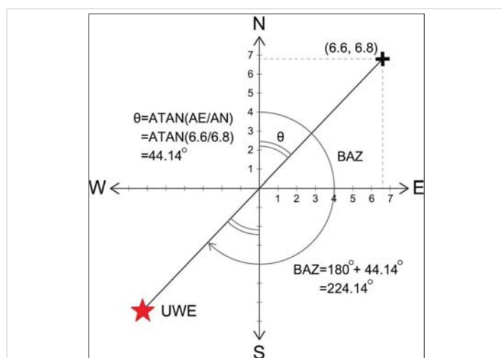
Figure 3: Determination of the direction of a site of the underwater explosion using the vector resultant of the first-arrival amplitudes (AN and AE) from two horizontal components of N-S and E-W and the positive motion of the first arrival on the vertical component. The positive first P-wave arrival on the vertical component means that the source is in the opposite to the station (+).
