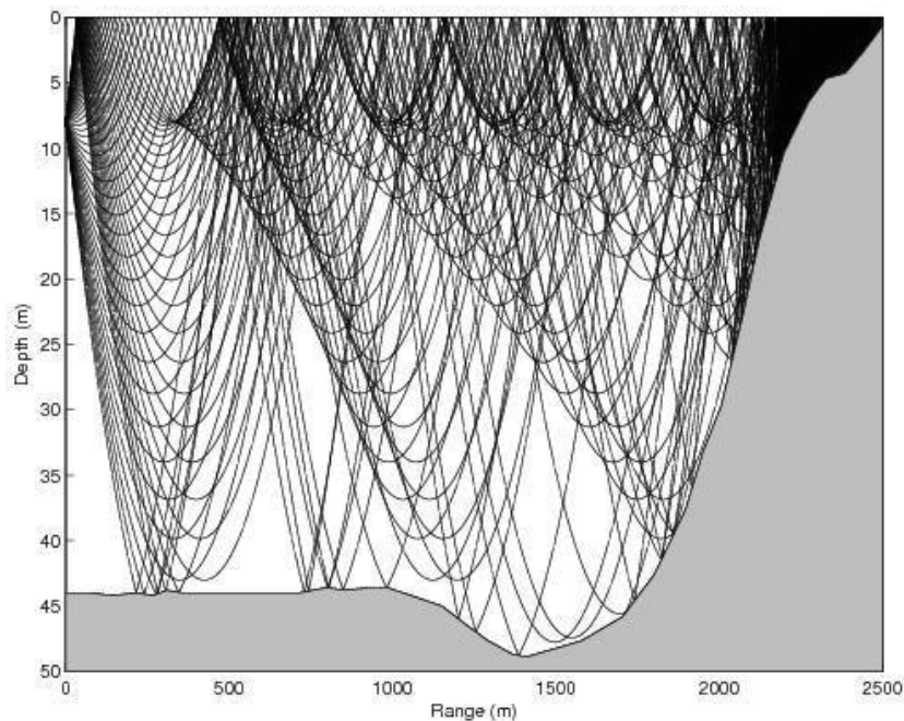
Figure 7: Ray-tracing based on hydroacoustic wave speed in the early spring season with a UWE source detonated at about 8 m offshore the Baengnyeong Island in the Yellow Sea. It exhibits shallow guided waves produced by total reflection of hydroacoustic waves from the free surface in the low-velocity layer at the subsurface and deep guided waves which are trapped by total reflection of hydroacoustic waves from the sea bottom [1-3].
