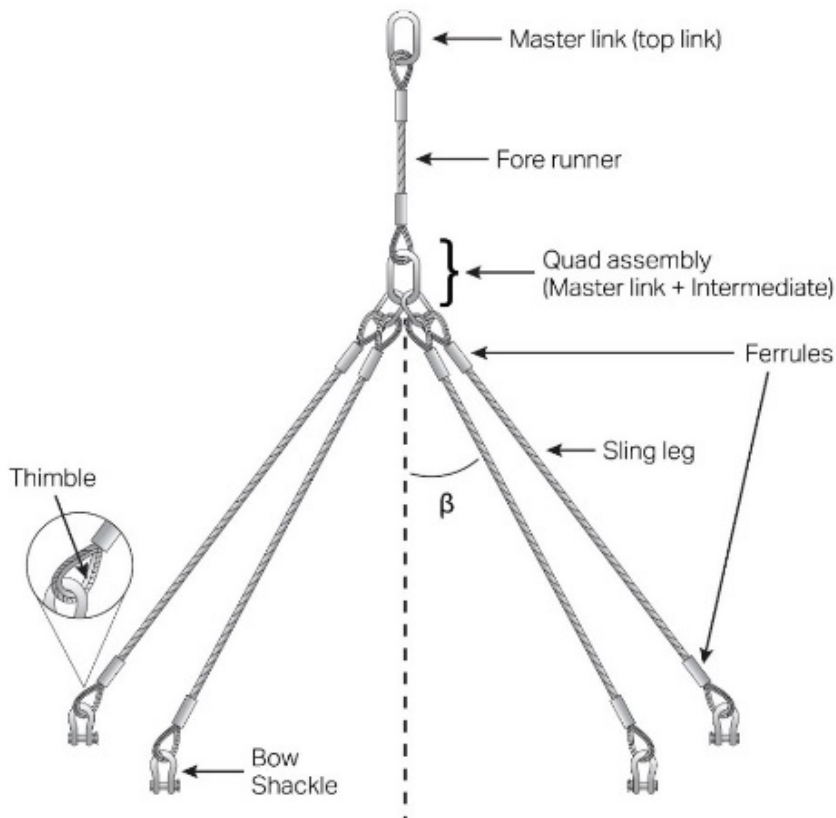
FIGURE 2 Four Legged Wire Sling with Fore Runner
