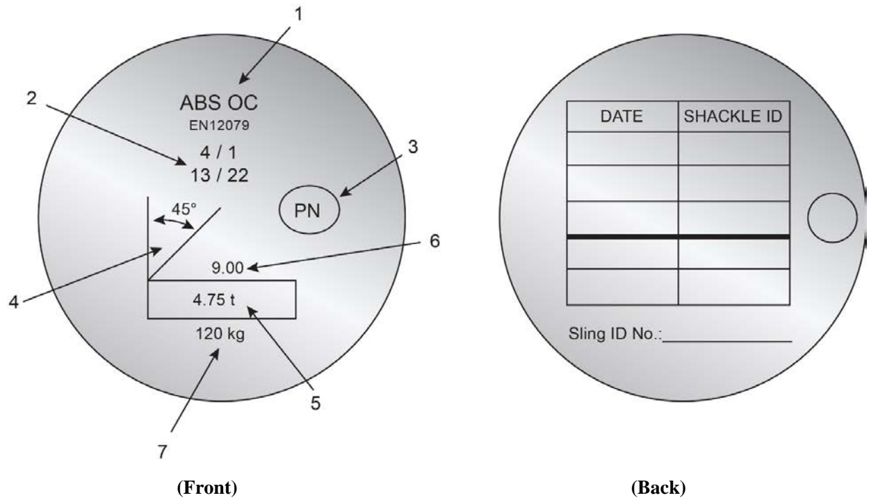
FIGURE 2 Identification Tag for Wire Rope Sling
