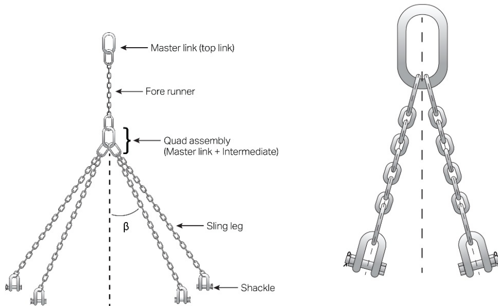
FIGURE 3 Chain Slings
