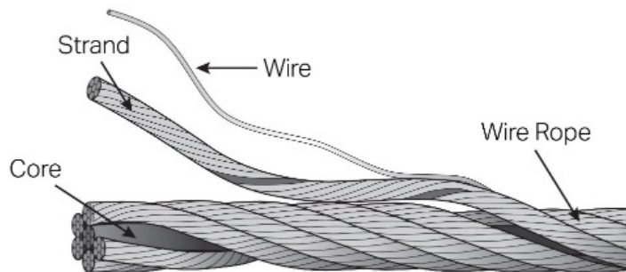
FIGURE 1 Construction of Wire Rope
