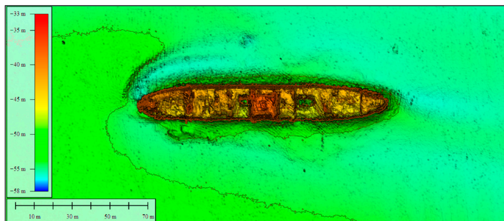
Figure 15. MBES survey of the Tilden wreck and bathymetry (courtesy of ISPRA, Astrea ).
