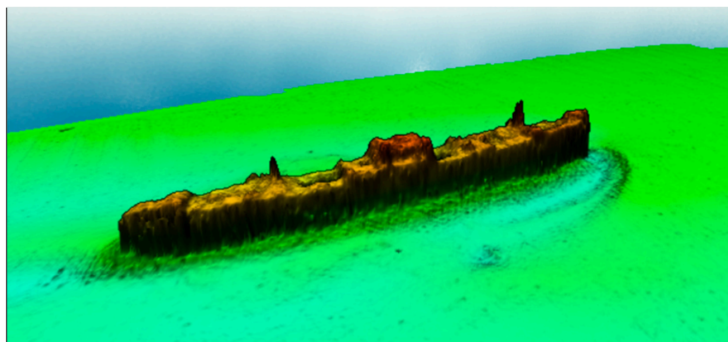
Figure 6. MBES survey of the Tilden wreck (courtesy of ISPRA, Astrea ).
