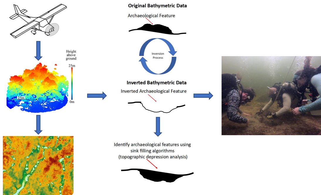
FIGURE 2 | Illustration of methods workflow. Bathymetric LiDAR was collected from a Cessna aircraft. The point data were then interpolated into a digital surface model (DSM). Next, we inverted the derived DSM to allow established topographic depression (or sink filling) algorithms to identify anthropogenic mound/midden anomalies present in the data. These detections were manually evaluated, and select sites were chosen for ground verification via SCUBA survey. Photo credit: Trevor Johnson.
