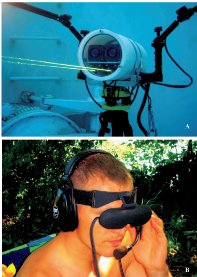
Fig. 11. System of three-dimensional visualisation of underwater objects: A – underwater part of the system during basin tests, two-camera system of picture acquisition in DVD quality, laser subsystem for placing background points to the frame to allow its scaling and dimensioning, B – element of surface part of the system – subsystem for head-located visualisation, operator is equipped with special goggles and receives a non-compressed picture from two cameras, to each eye separately [13].
