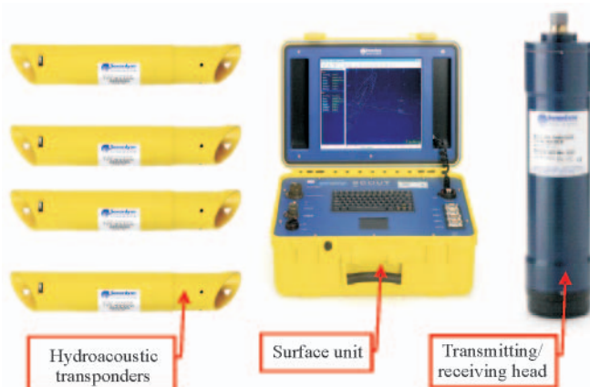
Fig. 4. Producer's set of the USBL Scout system
