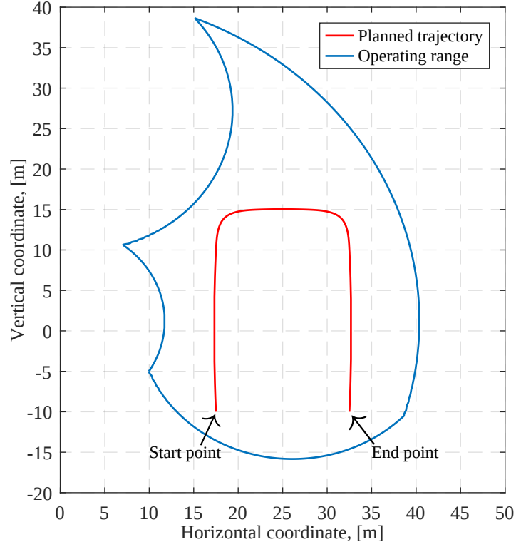
Figure 6: Planned trajectory within crane operating range.
