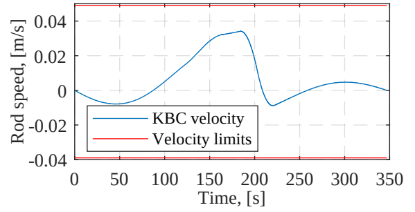
Figure 8: KBC velocity and limits.
