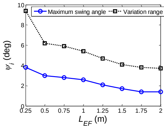
FIGURE 11. Effect of L_{EF} on the payload swing
