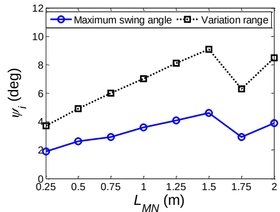
FIGURE 14. Effect of L_{MN} on the in-plane swing
