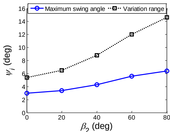
FIGURE 12. Effect of \beta_2 on the in-plane swing
