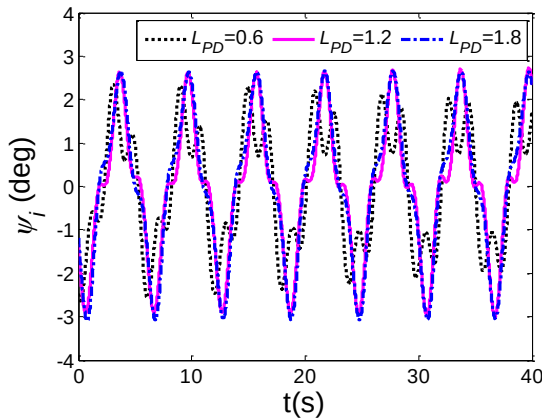
FIGURE 8. Effect of L_{PD} on the payload swing
