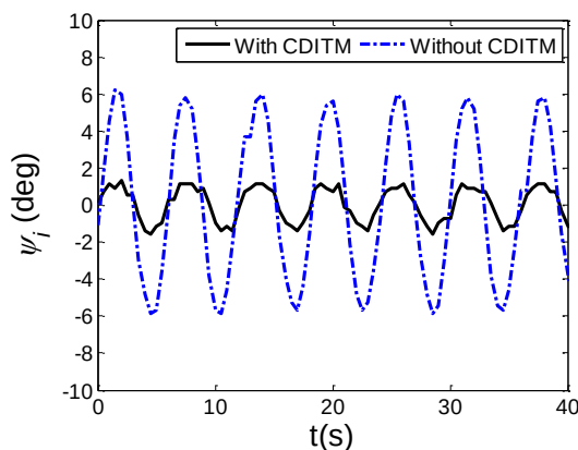
FIGURE 21. In-plane swing (With VS without CDITM, ship roll 4 deg)
