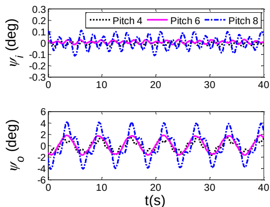
FIGURE 5. Effect of ship pitch on the payload swing
