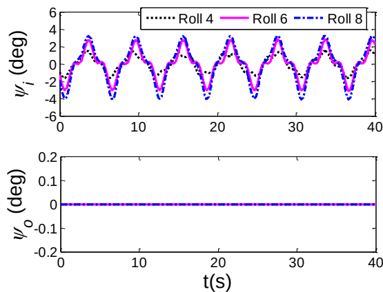
FIGURE 4. Effect of ship roll on the payload swing
