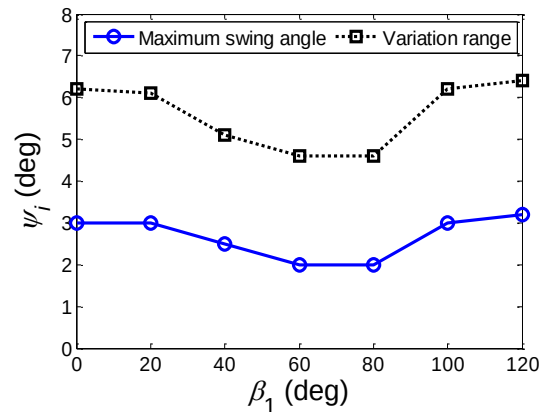
FIGURE 10. Effect of \beta_1 on the payload swing
