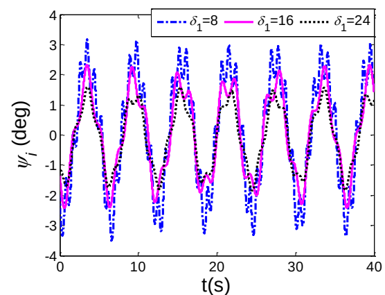
FIGURE 7. Effect of \delta_1 on the payload swing
