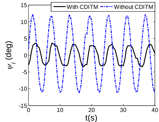
FIGURE 22. In-plane swing (With VS without CDITM, ship roll 8 deg)
