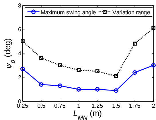
FIGURE 15. Effect of L_{MN} on the out-plane swing
