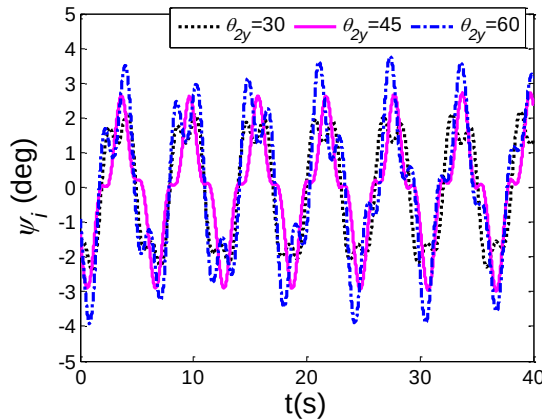
FIGURE 9. Effect of \theta_{2y} on the payload swing
