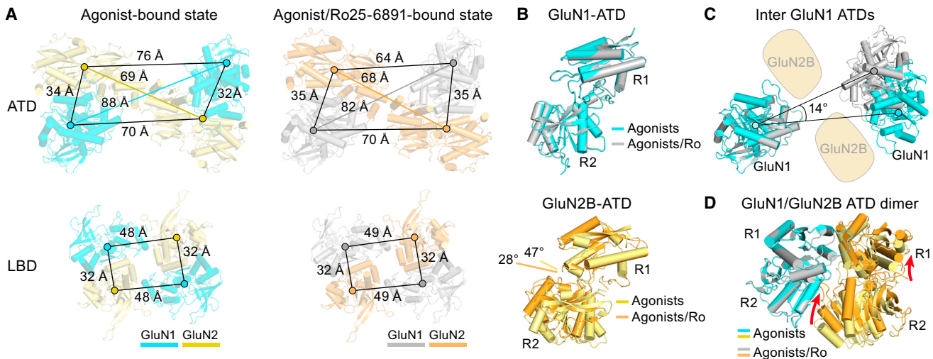
Figure 5. Conformational Changes Effected by Allosteric Inhibitor
