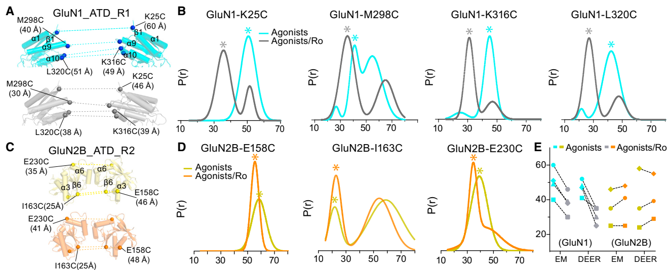
Figure 6. Separation of GluN1 ATDs but Not GluN2 ATDs, Detected by DEER
