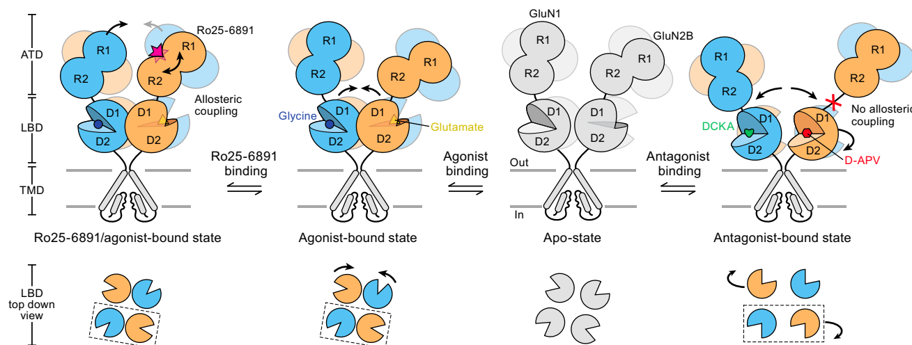
Figure 7. Schematic Summary of ECD Conformational Changes in NMDAR
