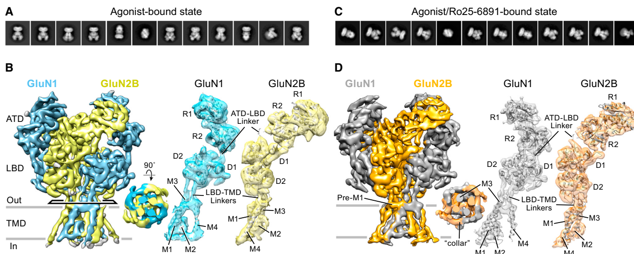
Figure 4. Cryo-EM Structures of Agonist- and Agonist/Ro25-6981-Bound Receptors
