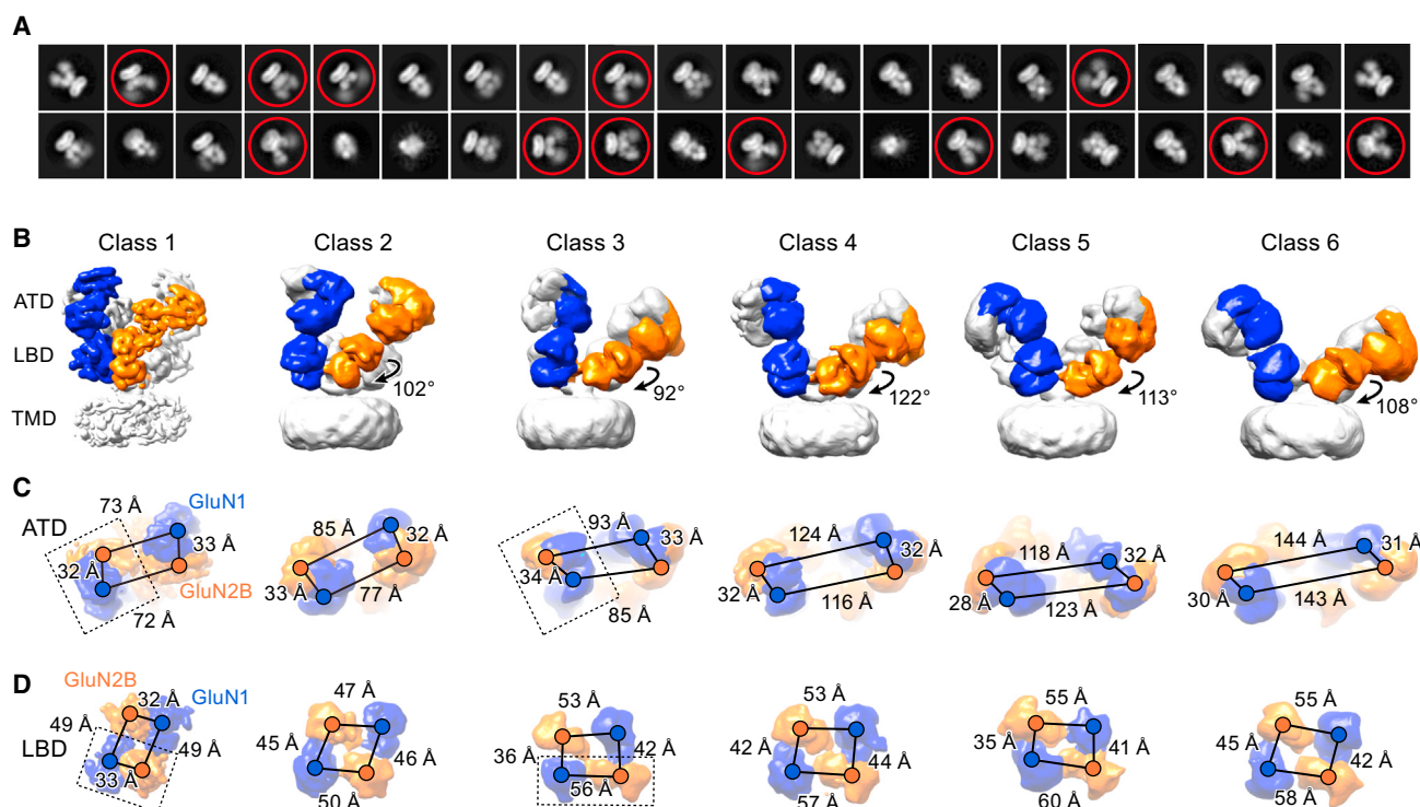
Figure 1. Cryo-EM Structures of Antagonist-Bound Receptors
