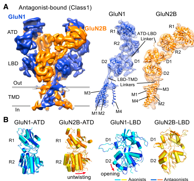
Figure 2. Competitive Antagonist Binding Induces Clamshell Conformational Changes
