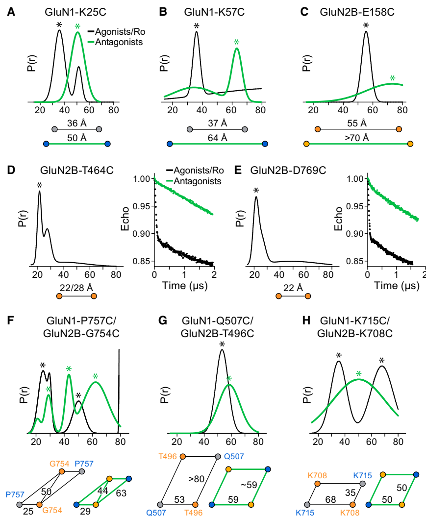
Figure 3. Conformational Changes in the Antagonist-Bound State Monitored by DEER
