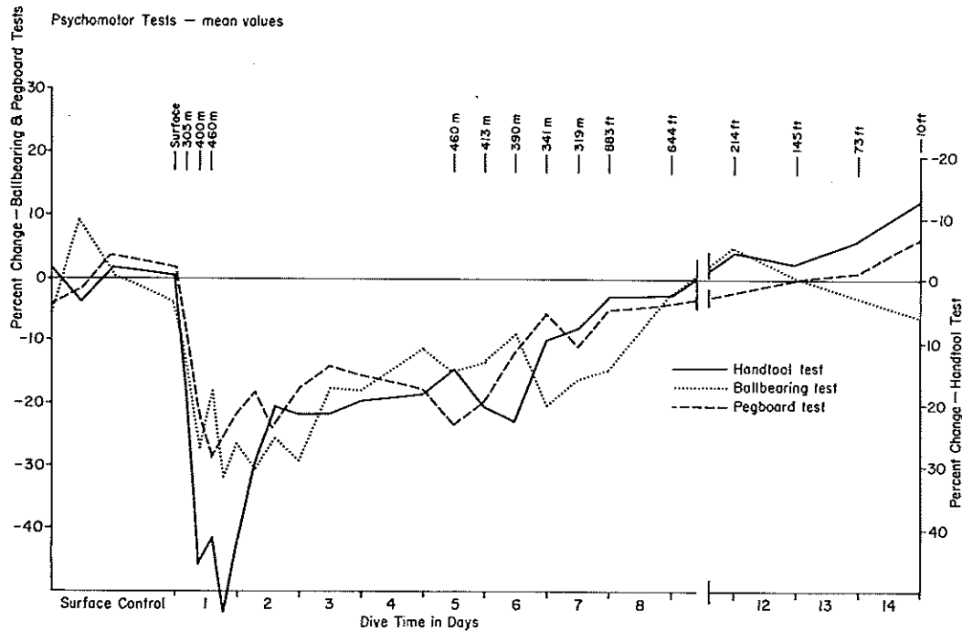
Fig. 4. Mean values of three subjects' psychomotor performance tests during Atlantis I exposure to 460 m (1509 ft) using 5% nitrogen in helium-oxygen and a compression time of 12 h 20 min.
