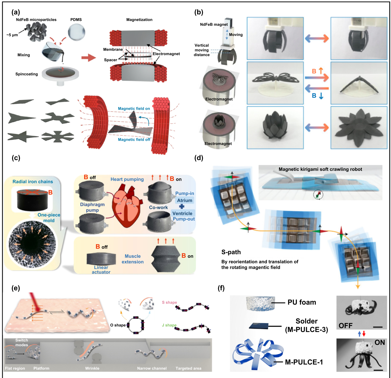
Figure 5. The magnetic-responsive actuators. (a) Schematic illustration of the driving mechanism of the magnetic-responsive actuator. Reproduced from [62]. CC BY 4.0. (b) Magnetic field-induced deformation of biomimetic magnetic actuators. Reprinted with permission from [72]. Copyright (2021) American Chemical Society. (c) Magnetically soft actuators with radial-chain iron microparticles for mimicking heart pumping and muscle extension. Reprinted with permission from [74]. Copyright (2021) American Chemical Society. (d) A magnetic kirigami robot that crawls in response to a rotating magnetic field. Reproduced from [76]. CC BY 4.0. (e) Magnetic millirobots with switchable locomotion modes negotiating complex barriers. Reprinted with permission from [81]. Copyright (2024) American Chemical Society. (f) Multifunctional and multi-material magnetic soft actuator with local controllability. Reproduced with permission from [82]. Copyright © 2022 The Authors, some rights reserved; exclusive licensee American Association for the Advancement of Science. No claim to original U.S. Government Works. Distributed under a Creative Commons Attribution NonCommercial License 4.0 (CC BY-NC).
