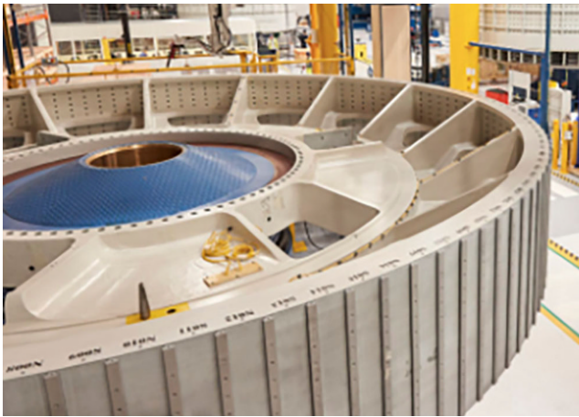
Fig. 13 Photo of GE's Haliade 6MW Rotor [32]
