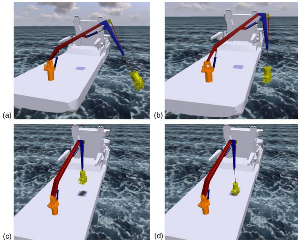
The operation started from the load recovering from the sea with a 45° load sway in the ship transverse direction a. Anti-sway control b and heave compensation applied before and during manoeuvring the load to the ship board c. Then the load was lifted up via the winch and lowered on the deck d
