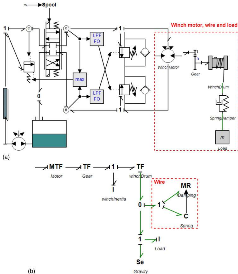
8 a Winch hydraulic sub-model and b bond graph (BG) of winch motor, wire and load
