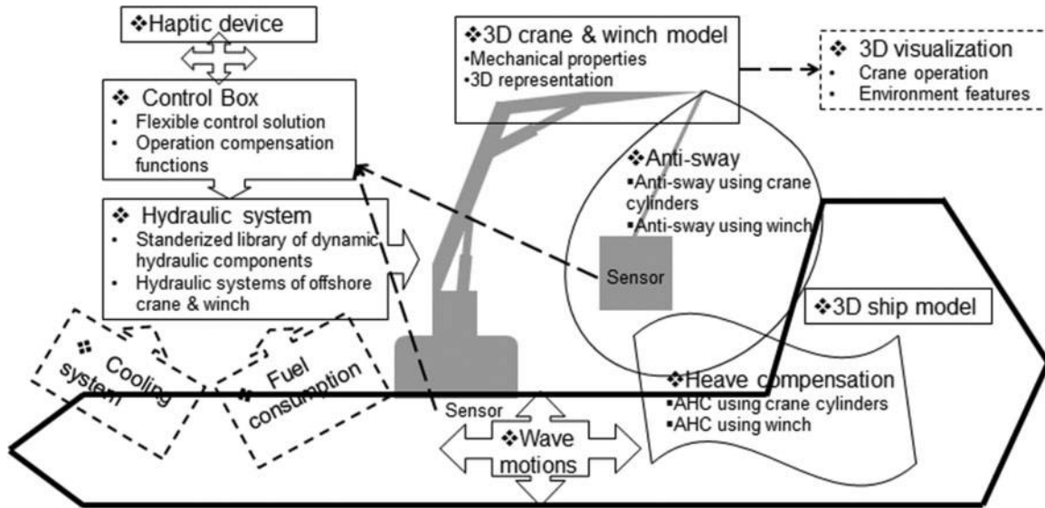
1 Offshore hydraulic crane modelling structure
