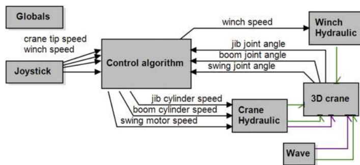
6 Crane control model – with hydraulics – without compensation functions
