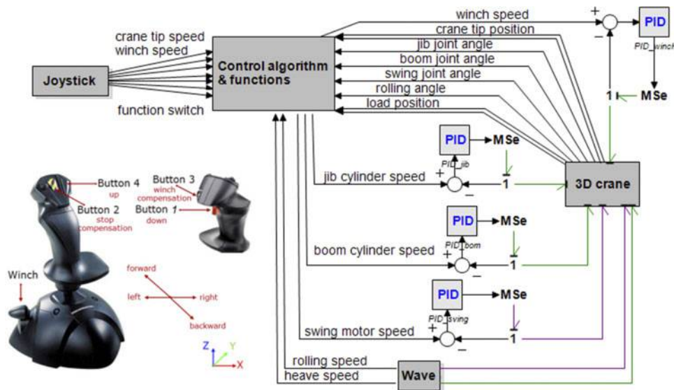
5 Crane control model – with compensation functions – without hydraulics
