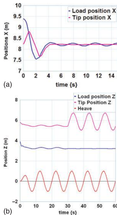
a Anti-sway; b heave compensation using crane and winch
