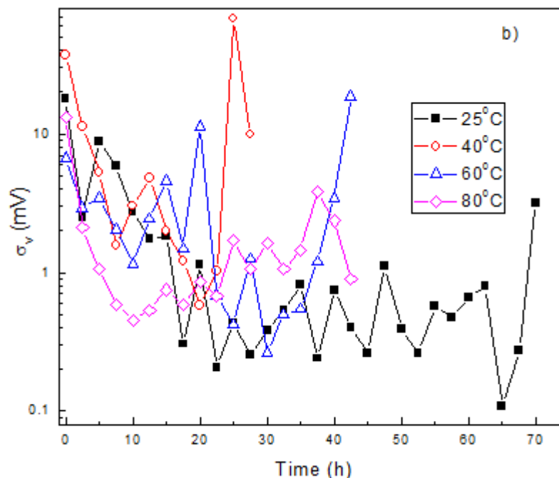
Figure 9. Variation with time of the a) current noise standard deviation, \sigma_i and b) potential noise standard deviation values, \sigma_v , for the different SSRT experiments.
