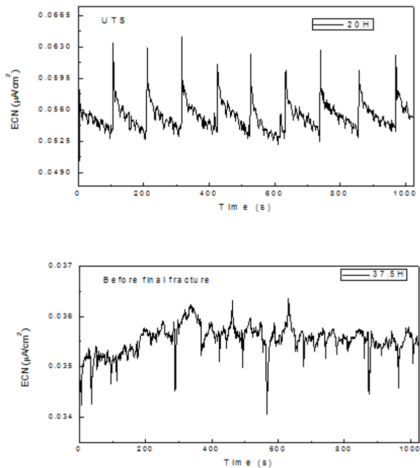
Figure 6. Noise in current for S41425 steel strained in the \text{H}_2\text{S} -containing 3.5% NaCl solution at 80^\circ\text{C} a) before straining, b) at the yielding pint, c) near the UTS and d) before final fracture.
