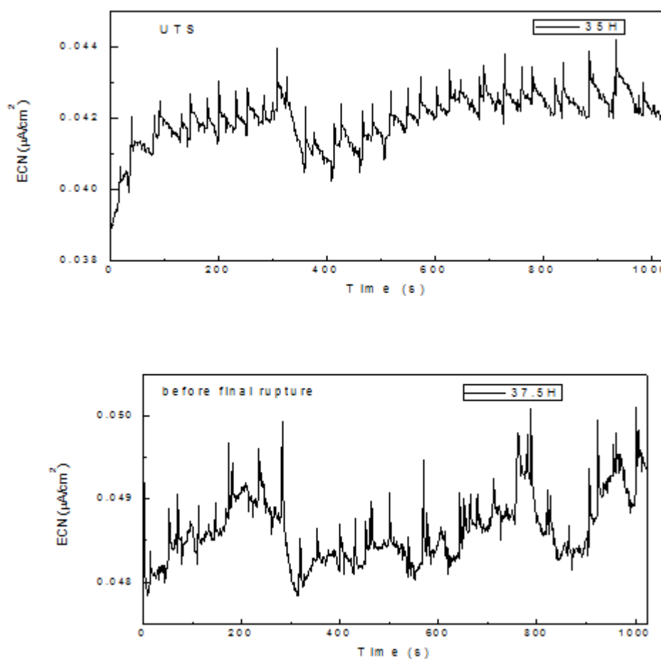
Figure 4. Noise in current for S41425 steel in strained in the H 2 S-containing 3.5% NaCl solution at 60 °C a) before straining, b) at the yielding point, c) near the UTS and d) before final fracture.
