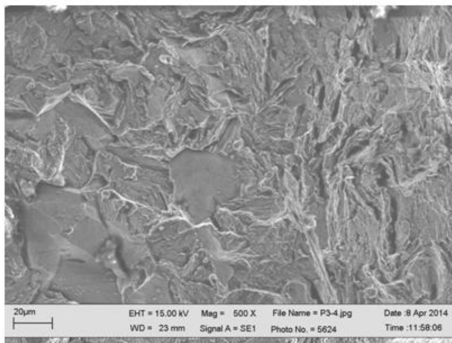
Figure 5. SEM micrograph of S41425 steel fractured in the H 2 S-containing 3.5% NaCl solution at 60°C
