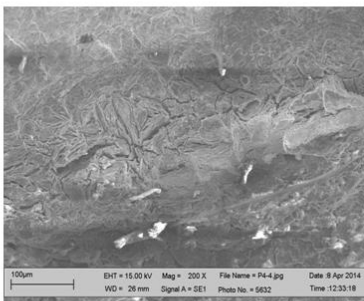
Figure 7. SEM micrograph of S41425 steel fractured in the \text{H}_2\text{S} -containing 3.5% NaCl solution at 80^\circ\text{C} .
