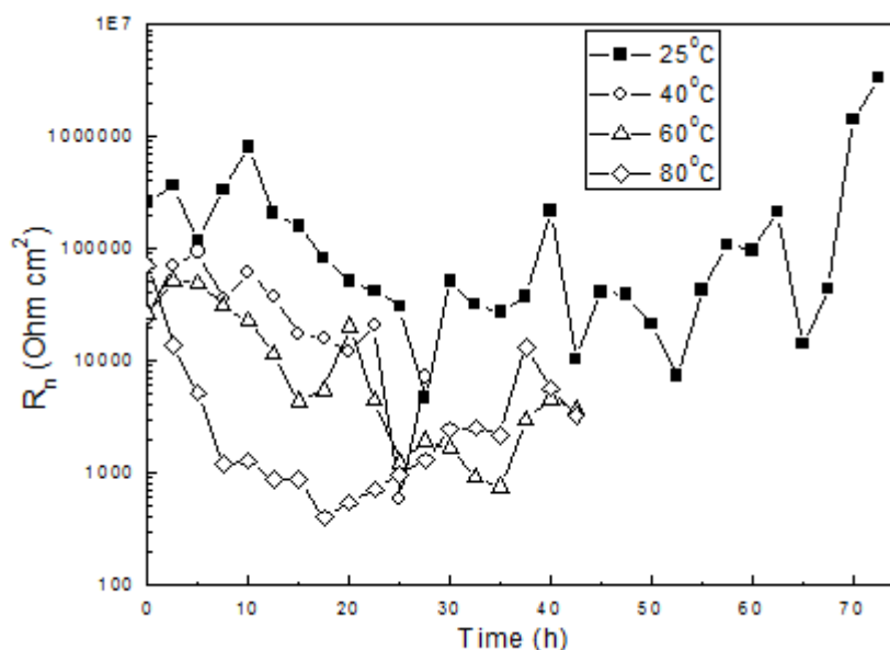
Figure 10. Variation of the noise resistance value, R_n , with time for the different SSRT experiments.
