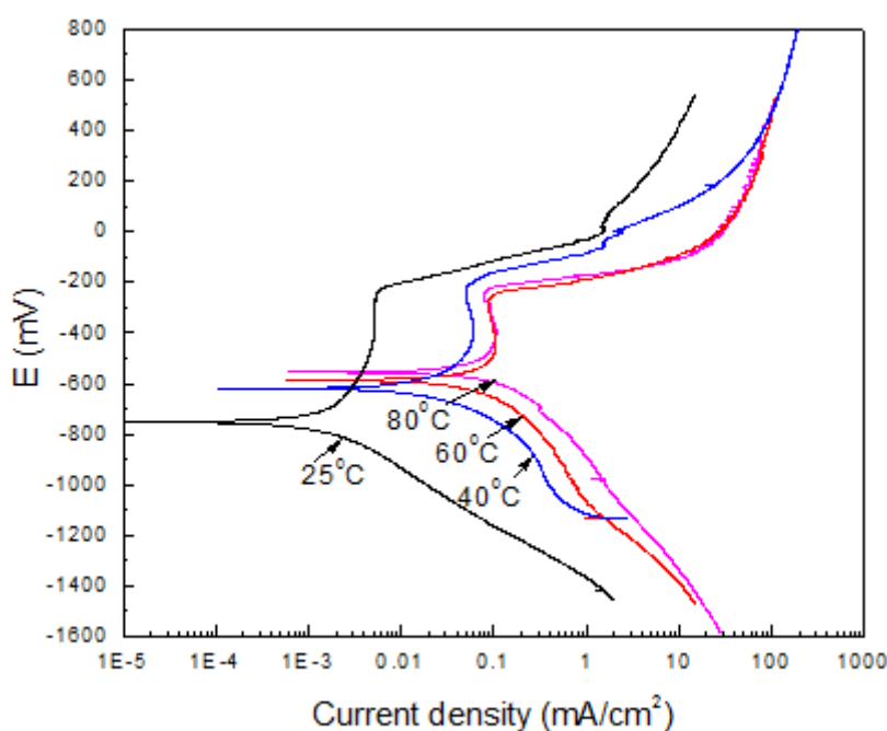
Figure 1. Effect of the temperature in the polarization curves for S41425 in a \text{H}_2\text{S} -containing 3.5% NaCl solution.
