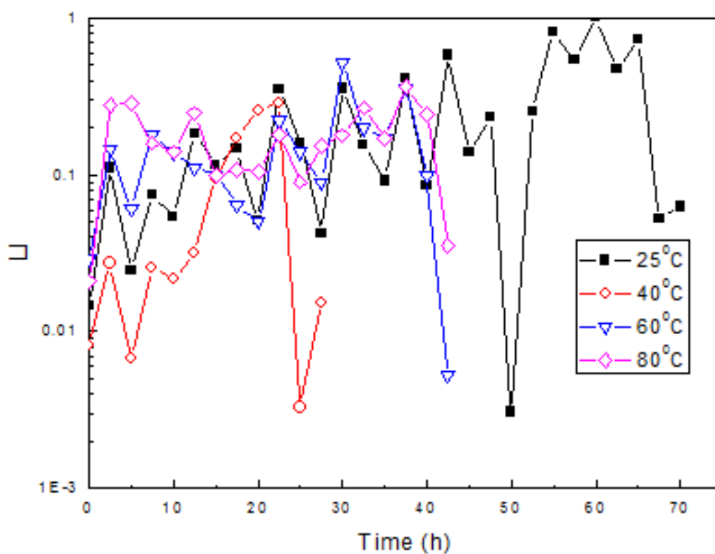
Figure 8. Variation of the localization index value, LI, with time for the different SSRT experiments.
