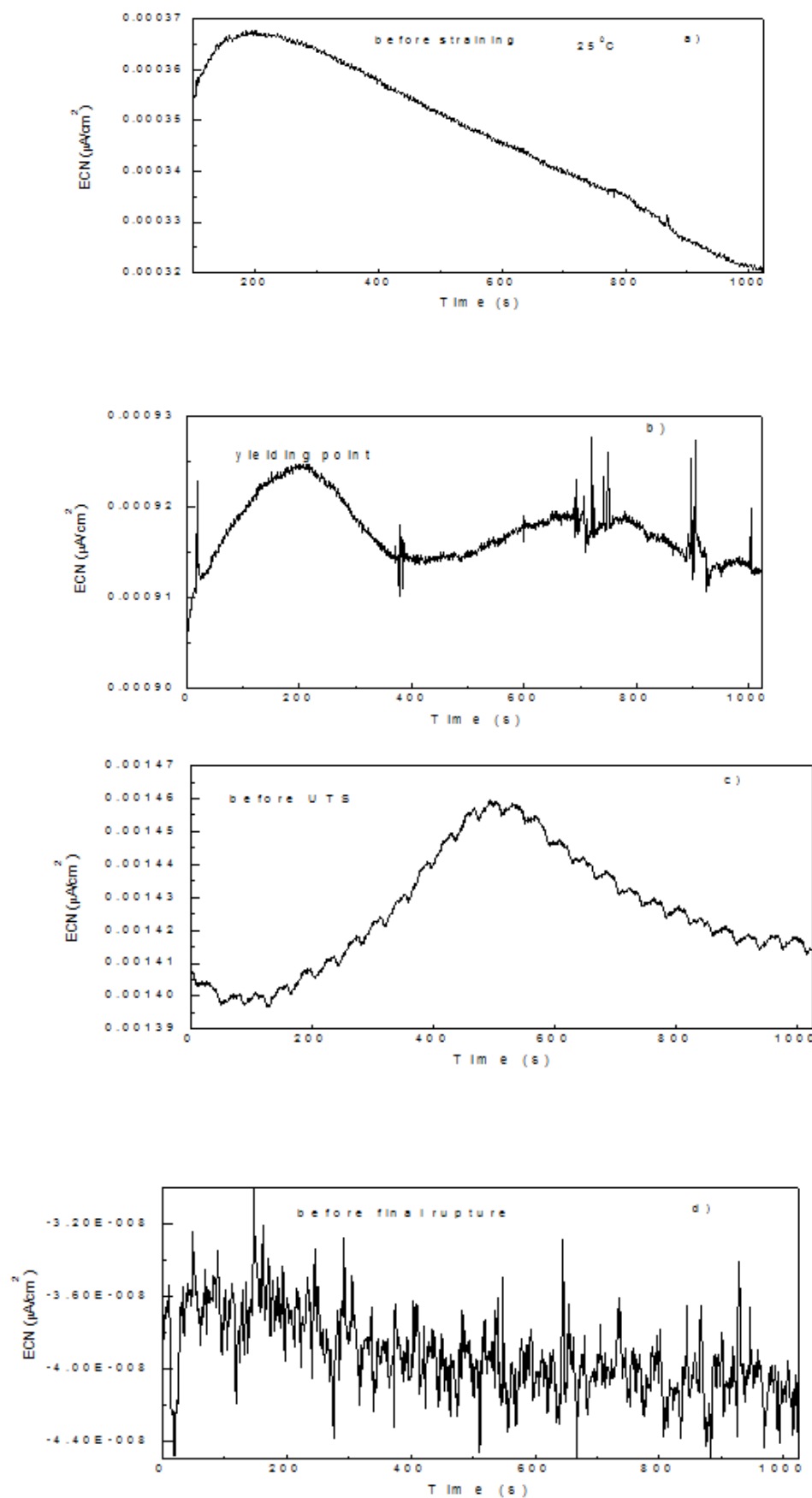
Figure 2. Noise in current for S41425 steel in the \text{H}_2\text{S} -containing 3.5% NaCl solution at 25^\circ\text{C} a) before straining, b) at the yielding point, c) near the UTS and d) before final fracture.
