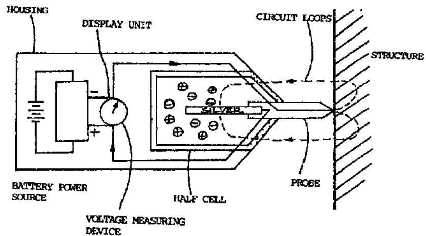
Simple schematic of a bathyconrometer:
