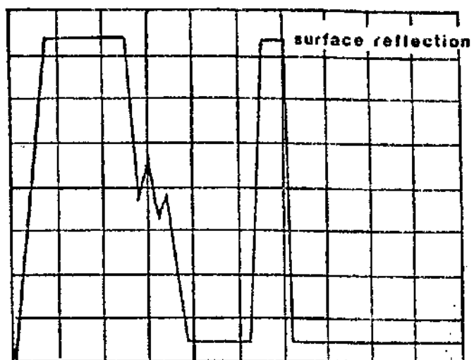
(3) GOOD PROBE CONTACT - PARTIALLY FLOODED Rovprobe, Cathode Ray Tube Displays.
