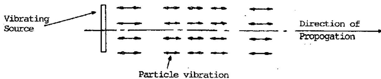
Compression waves
