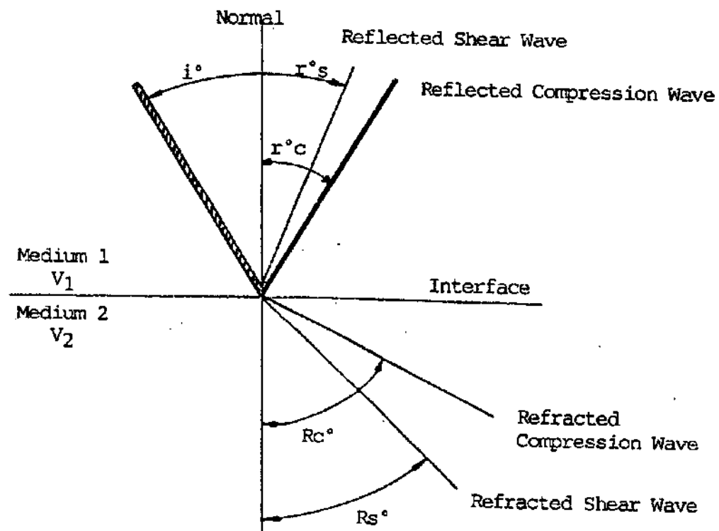
Reflection and Refraction: Snells Law
