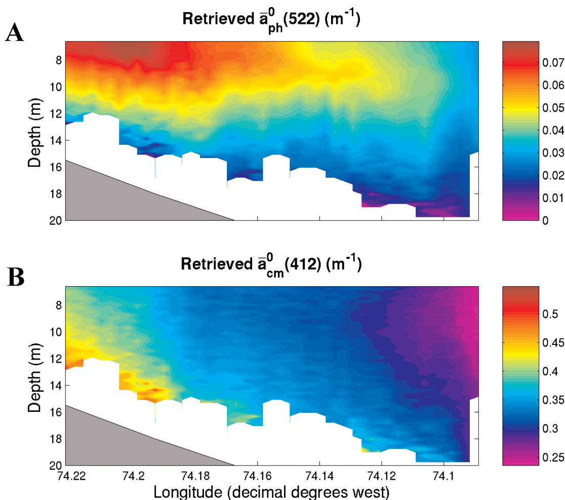
Fig. 9. Inverse model results for \delta\bar{K}_d^0(\lambda, z_{AUV}) along the A-line transect (Method 2). (A) Retrieved average absorption by phytoplankton ( \bar{a}_{ph}^0(522) ; m^{-1} ). (B) Retrieved absorption by nonalgal colored matter at 412 nm ( \bar{a}_{cm}^0(412) ; m^{-1} ).
