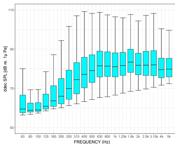
Figure 9: Statistics of ship traffic sounds in LIIVI 02 site. Exceedance levels L_{75} and L_{25} are indicated by the lower and upper hinges of the boxplot while middle lines show the median values. The upper and lower whiskers indicate the 1.5 times difference of exceedance levels L_{25} and L_{75} . The figure is adapted from Publication 1.
