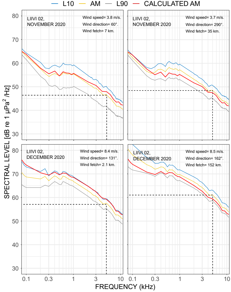
Figure 5: Comparison of measured AM wind-driven spectral levels for two contrasting wind fetches in the LIIVI 02 site. The calculated wind-driven spectral level considering all wind directions in the respective months was presented in the solid red lines. The spectral levels that might coincide with the high self-noise of the recorder are indicated with dash-dotted lines. The figure is adapted from Publication III.
