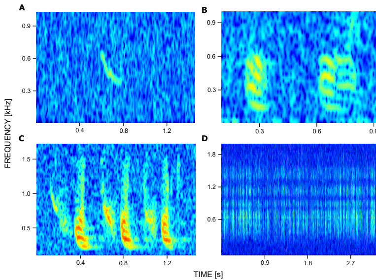
Figure 7: Spectrograms of underwater ringed seals' vocalisations A) yelp, B) bark C) alternating series of barks and yelp and D) scratches of ice by ringed seals. The figures are adapted from Publication I.
