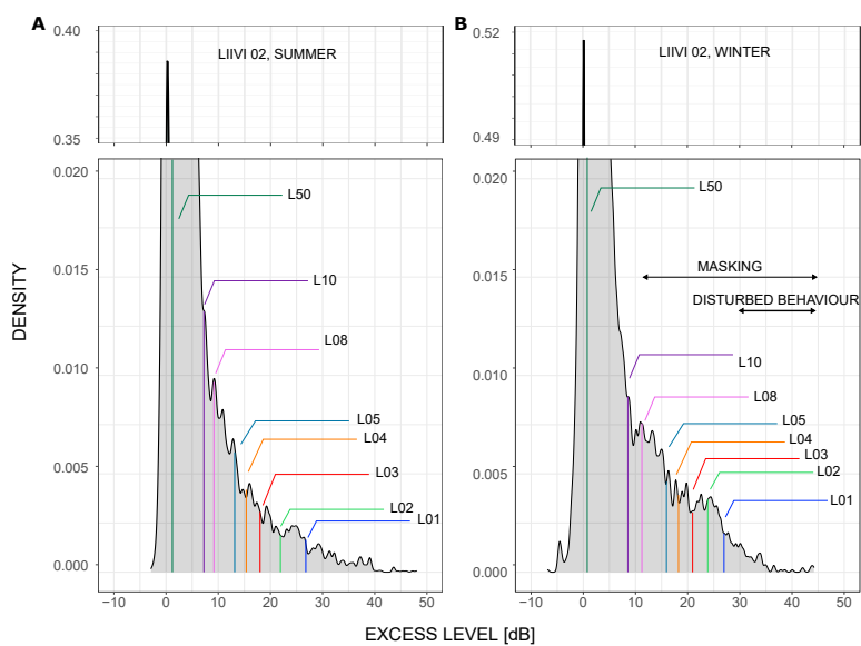
Figure 17: Weekly probability of excessive sound level at 500 Hz regarding the estimated LOBE value in the LIIVI 02 site. The figures are adapted from Publication 1.
