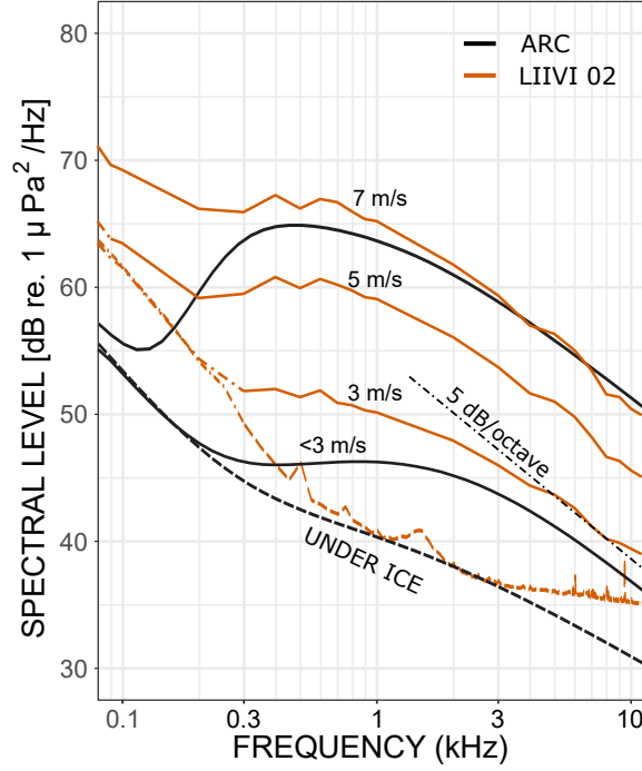
Figure 4: Wind-driven sound characteristics in the LIIVI O2 site (orange lines) and in the Finnish ARC site in GoF (black lines) [22]. At higher frequencies, a spectral slope of -5 dB/octave (dot-dashed line) appears. The sound levels measured under ice are shown as dashed lines. The figure is adapted from Publication III.
